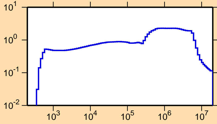
\sigma vs. E for ^{102}\text{Nb}(n,\text{inel.})
