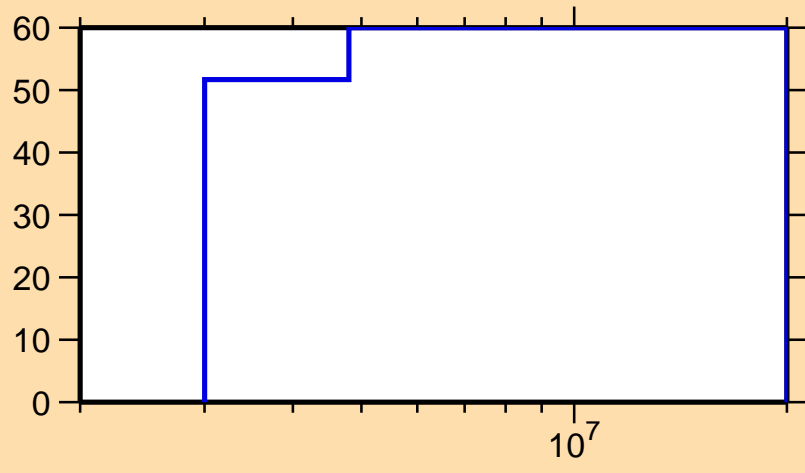
\Delta\sigma/\sigma vs. E for ^{102}\text{Nb}(n,\gamma)
