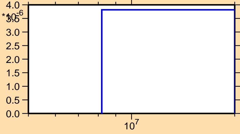
\sigma vs. E for ^{102}\text{Nb}(n,n\alpha)
