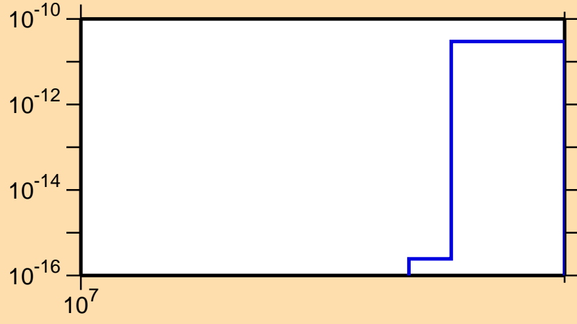
\sigma vs. E for ^{103}\text{Nb}(n,2n\alpha)
