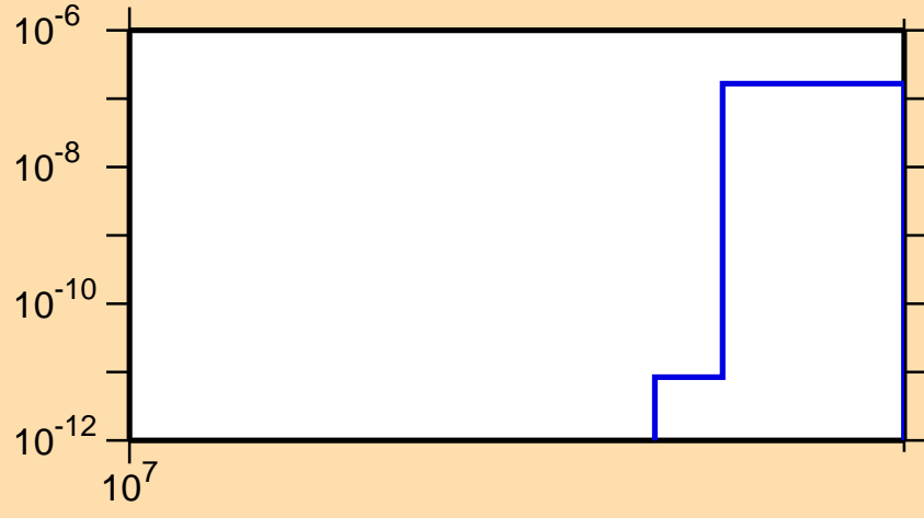
\sigma vs. E for ^{103}\text{Nb}(n,\text{nd})
