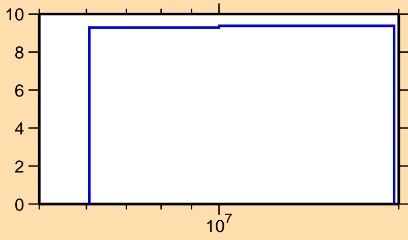
\Delta\sigma/\sigma vs. E for ^{103}\text{Nb}(n,\text{nonel.})
