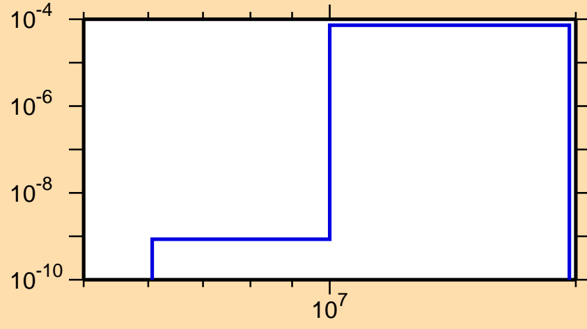
\sigma vs. E for ^{103}\text{Nb}(n,\alpha)
