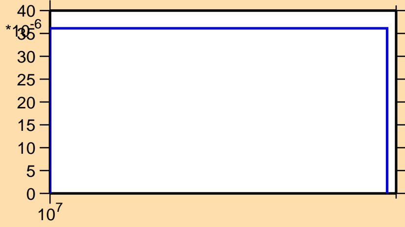
\sigma vs. E for ^{103}\text{Nb}(n,np)
