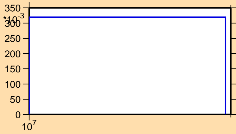
\sigma vs. E for ^{103}\text{Nb}(n,3n)
