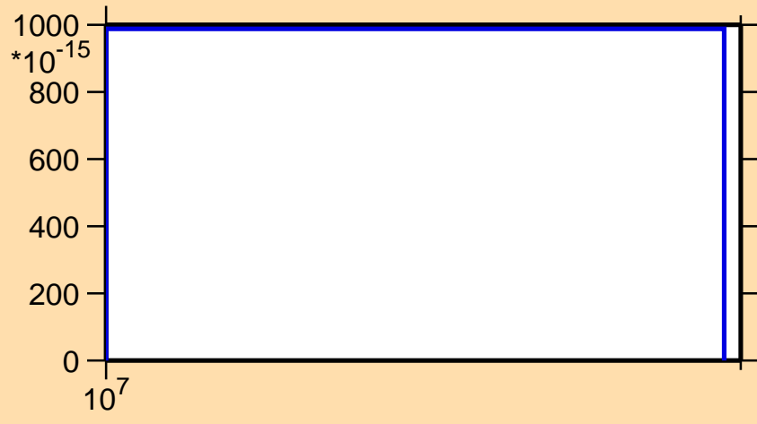
\sigma vs. E for ^{103}\text{Nb}(n,2np)
