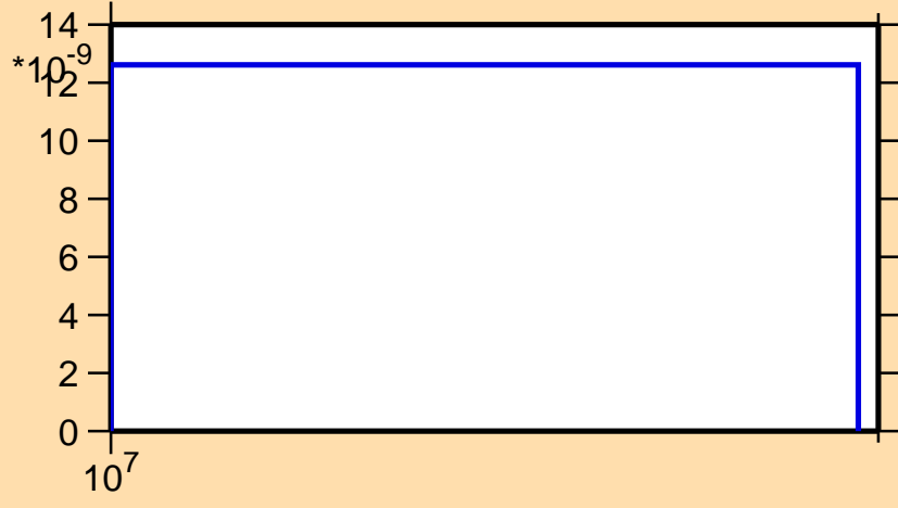
\sigma vs. E for ^{103}\text{Nb}(n,nt)
