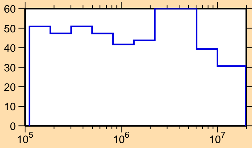
\Delta\sigma/\sigma vs. E for ^{103}\text{Nb}(n,n_1)
