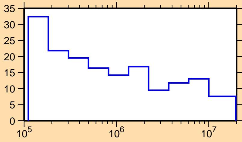
\Delta\sigma/\sigma vs. E for ^{103}\text{Nb}(n,\text{el.})
