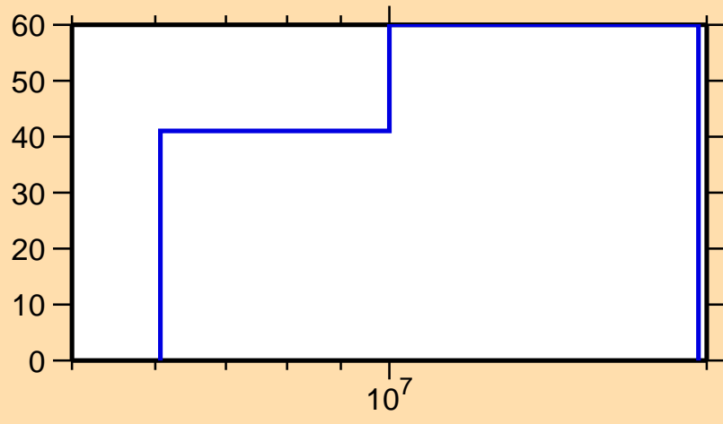
\Delta\sigma/\sigma vs. E for ^{103}\text{Nb}(n,n\text{cont.})
