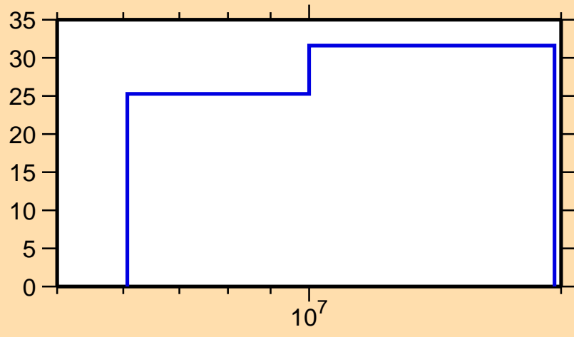
\Delta\sigma/\sigma vs. E for ^{103}\text{Nb}(n,\text{inel.})
