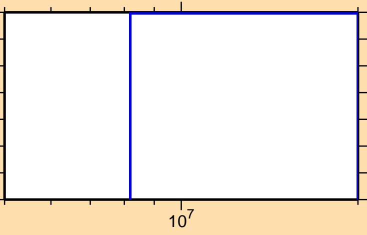
\sigma vs. E for ^{103}\text{Nb}(n,t)
