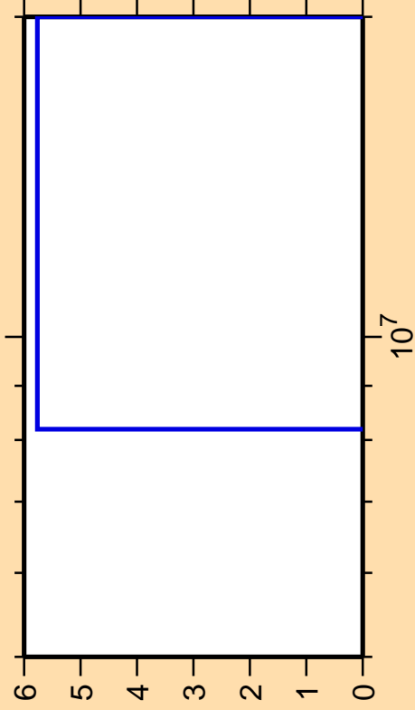
\Delta\sigma/\sigma vs. E for ^{103}\text{Nb}(n,2np)
