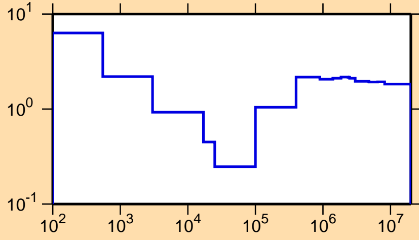
\sigma vs. E for ^{103}\text{Nb}(n,\text{nonel.})
