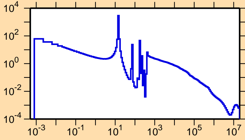
\sigma vs. E for ^{104}\text{Nb}(n,\gamma)
