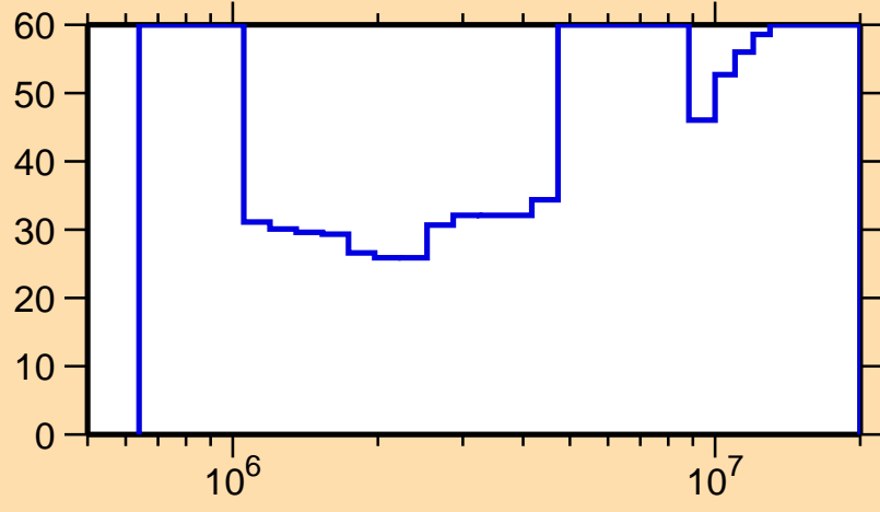
\Delta\sigma/\sigma vs. E for ^{104}\text{Nb}(n,n\text{cont.})
