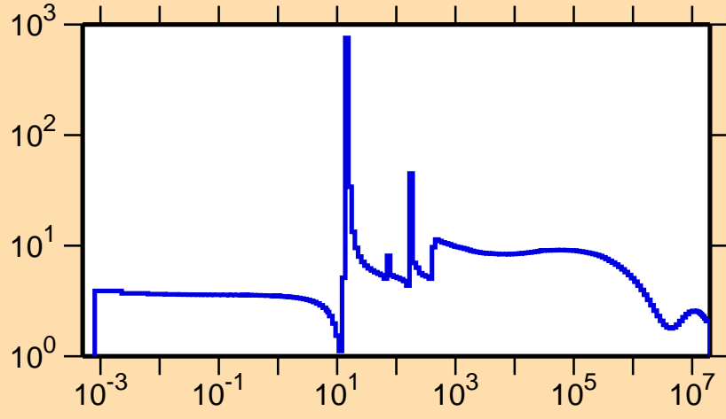
\sigma vs. E for ^{104}\text{Nb}(n,\text{el.})
