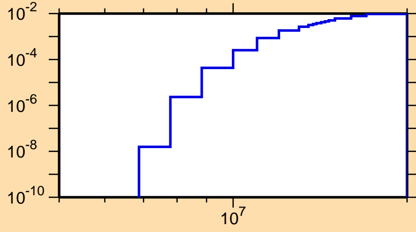
\sigma vs. E for ^{104}\text{Nb}(n,p)
