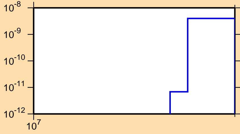
\sigma vs. E for ^{104}\text{Nb}(n,2n\alpha)
