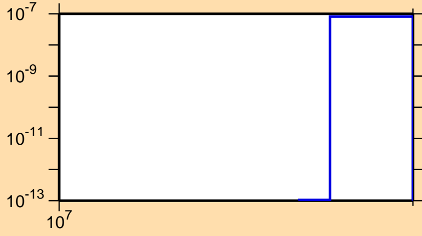
\sigma vs. E for ^{104}\text{Nb}(n,2np)
