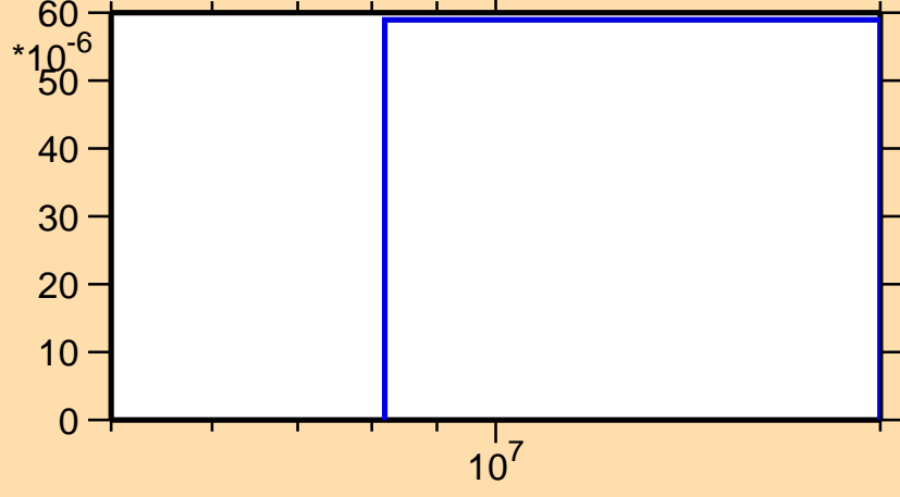
\sigma vs. E for ^{104}\text{Nb}(n,d)
