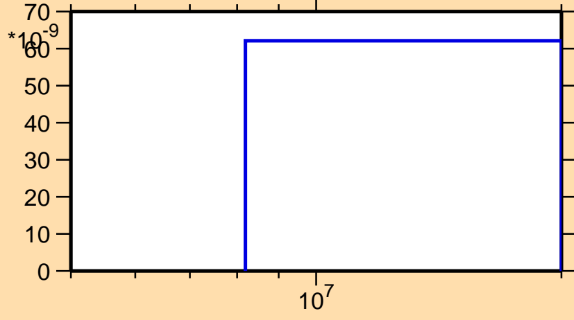
\sigma vs. E for ^{104}\text{Nb}(n,\text{nd})
