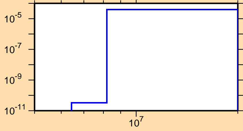
\sigma vs. E for ^{104}\text{Nb}(n,\alpha)
