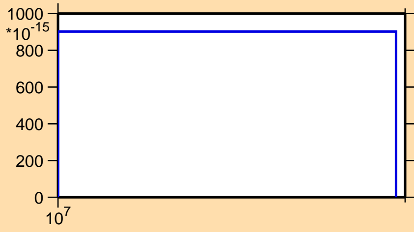
\sigma vs. E for ^{105}\text{Nb}(n,2np)
