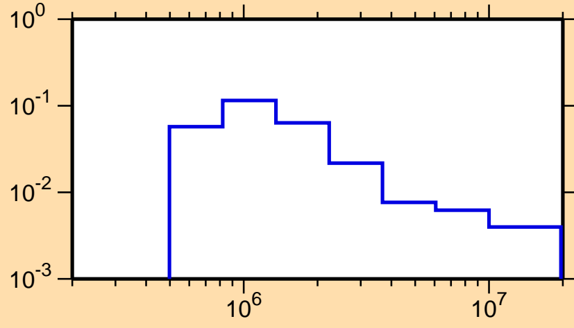
\sigma vs. E for ^{105}\text{Nb}(n,n_3)
