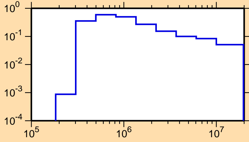
\sigma vs. E for ^{105}\text{Nb}(n,n_2)
