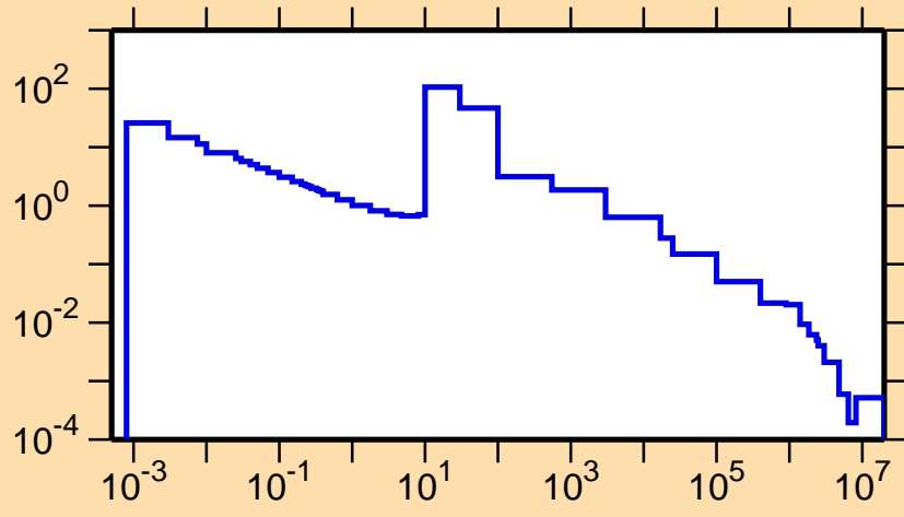
\sigma vs. E for ^{105}\text{Nb}(n,\gamma)
