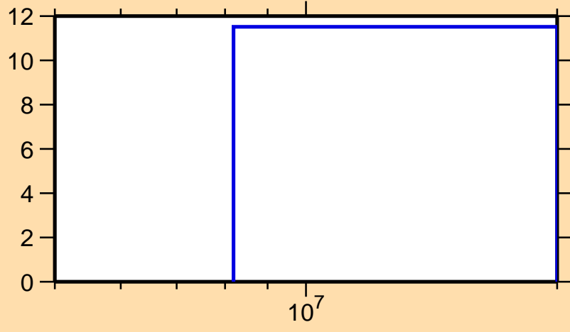
\Delta\sigma/\sigma vs. E for ^{105}\text{Nb}(n,el.)
