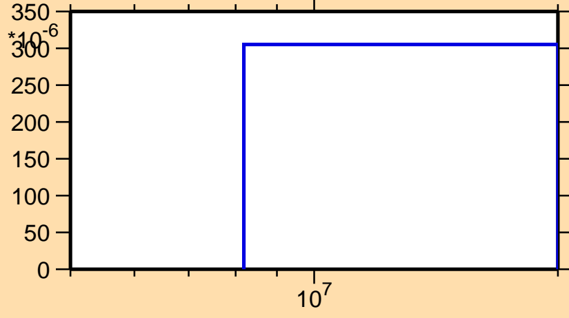
\sigma vs. E for ^{105}\text{Nb}(n,p)
