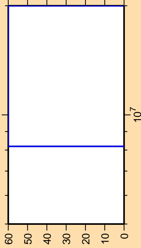
\Delta\sigma/\sigma vs. E for ^{105}\text{Nb}(n,nd)
