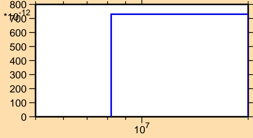
\sigma vs. E for ^{105}\text{Nb}(n,nd)
