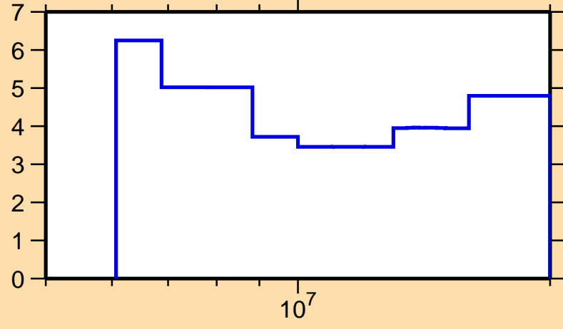
\Delta\sigma/\sigma vs. E for ^{106}\text{Nb}(n,\text{nonel.})
