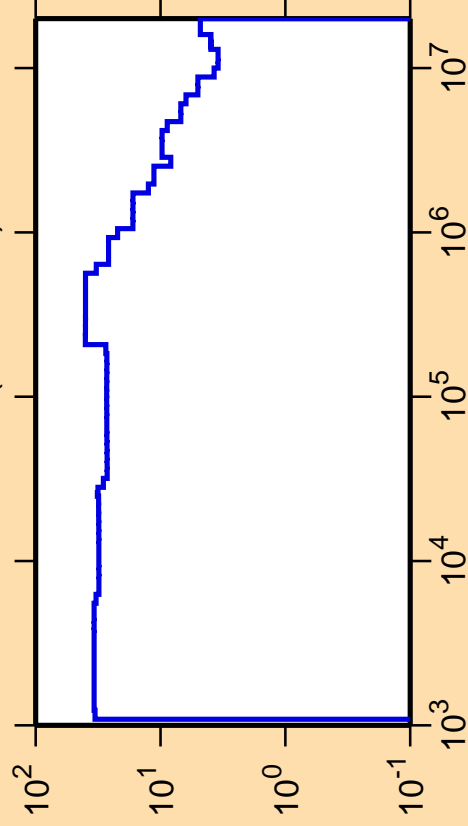
\Delta\sigma/\sigma vs. E for ^{106}\text{Nb}(n,\text{nonel.})
