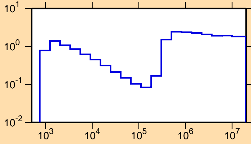
\sigma vs. E for ^{106}\text{Nb}(n,\text{nonel.})
