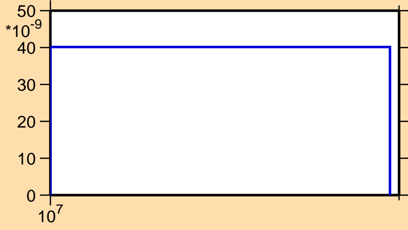
\sigma vs. E for ^{106}\text{Nb}(n,nd)
