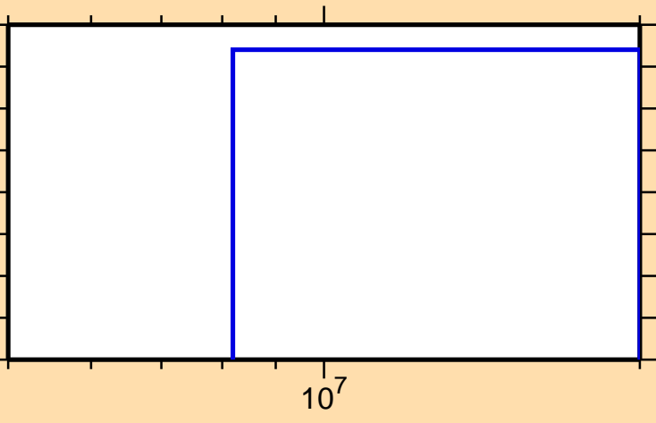
\sigma vs. E for ^{106}\text{Nb}(n,\text{nd})
