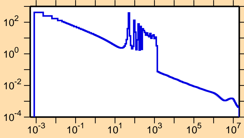
\sigma vs. E for ^{126}\text{Nd}(n,\gamma)
