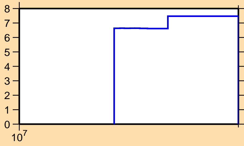
\Delta\sigma/\sigma vs. E for ^{126}\text{Nd}(n,\text{nonel.})
