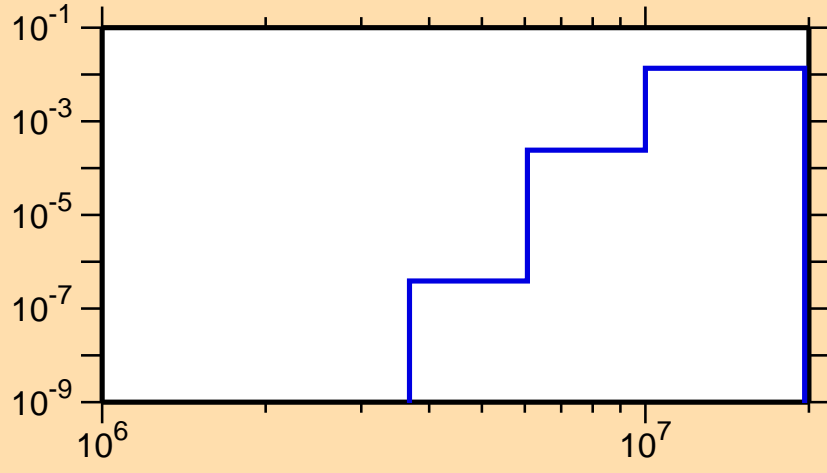
\sigma vs. E for ^{126}\text{Nd}(n,d)
