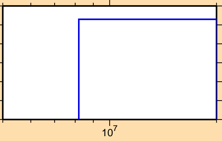
\sigma vs. E for ^{126}\text{Nd}(n,2np)
