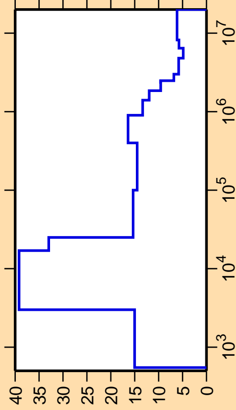
\Delta\sigma/\sigma vs. E for ^{126}\text{Nd}(n,\text{nonel.})
