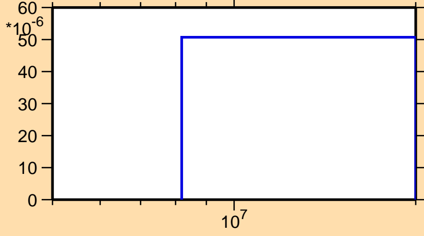
\sigma vs. E for ^{126}\text{Nd}(n,t)
