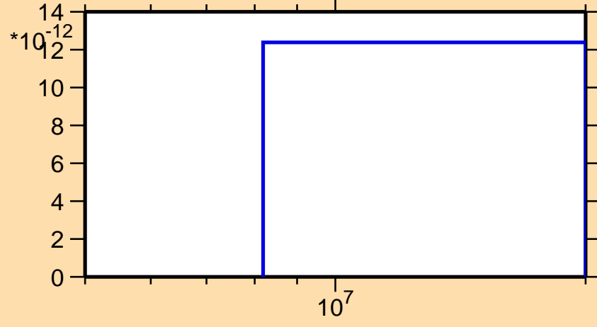
\sigma vs. E for ^{126}\text{Nd}(\text{mt } 34)
