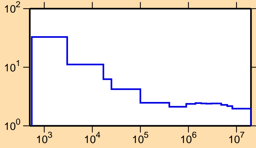
\sigma vs. E for ^{126}\text{Nd}(n,\text{nonel.})
