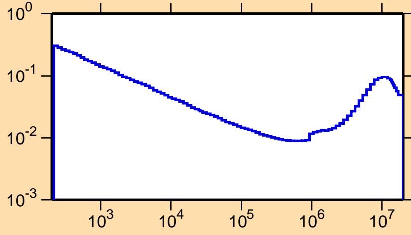
\sigma vs. E for ^{127}\text{Nd}(n,\alpha)
