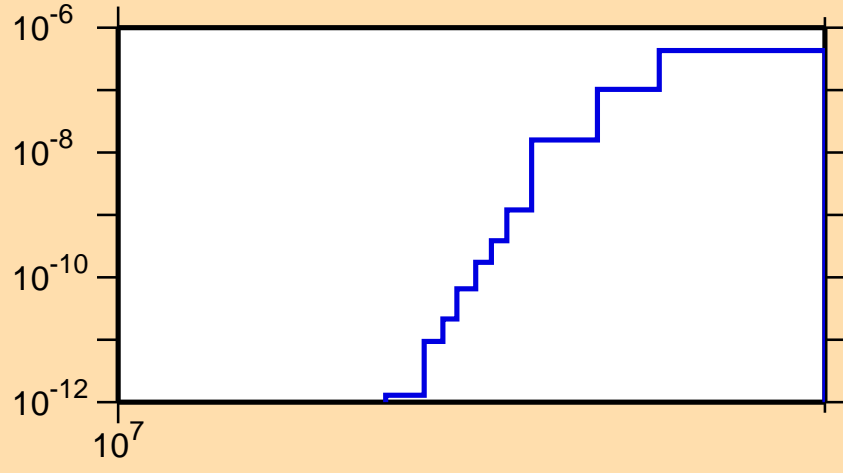
\sigma vs. E for ^{127}\text{Nd}(n,2n\alpha)
