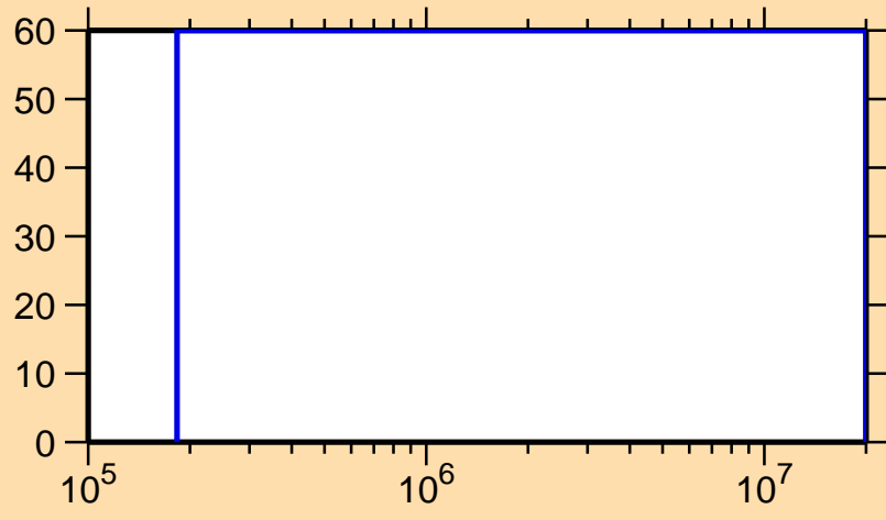
\Delta\sigma/\sigma vs. E for ^{127}\text{Nd}(n,n\text{cont.})
