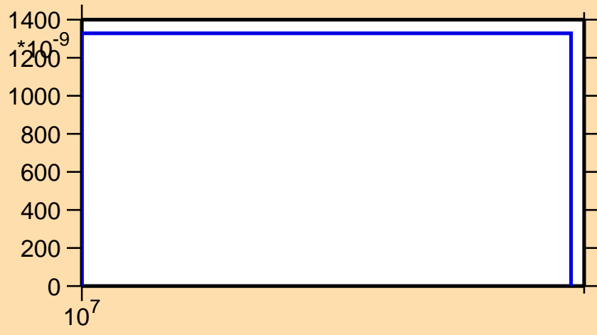
\sigma vs. E for ^{127}\text{Nd}(n,2np)
