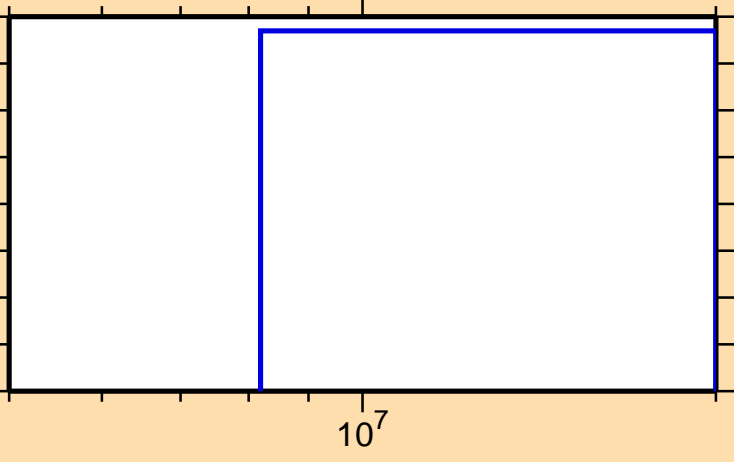
\sigma vs. E for ^{127}\text{Nd}(\text{mt } 34)
