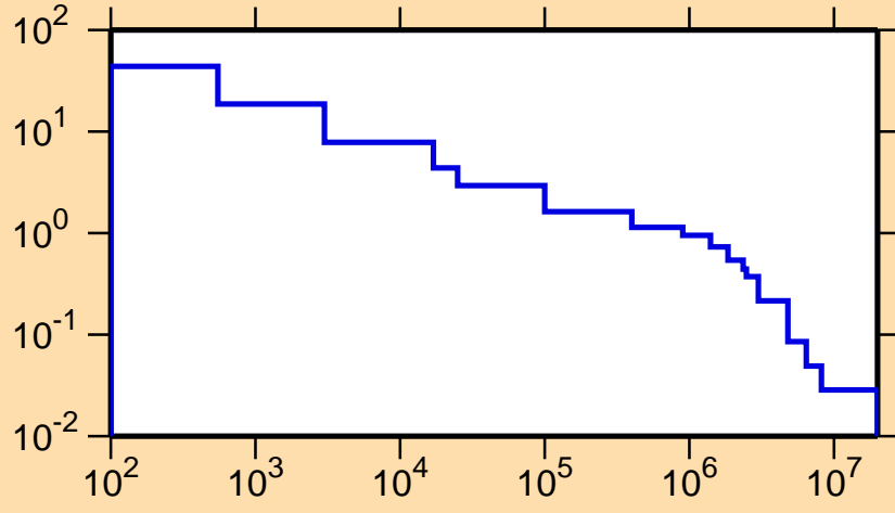
\sigma vs. E for ^{127}\text{Nd}(n,p)
