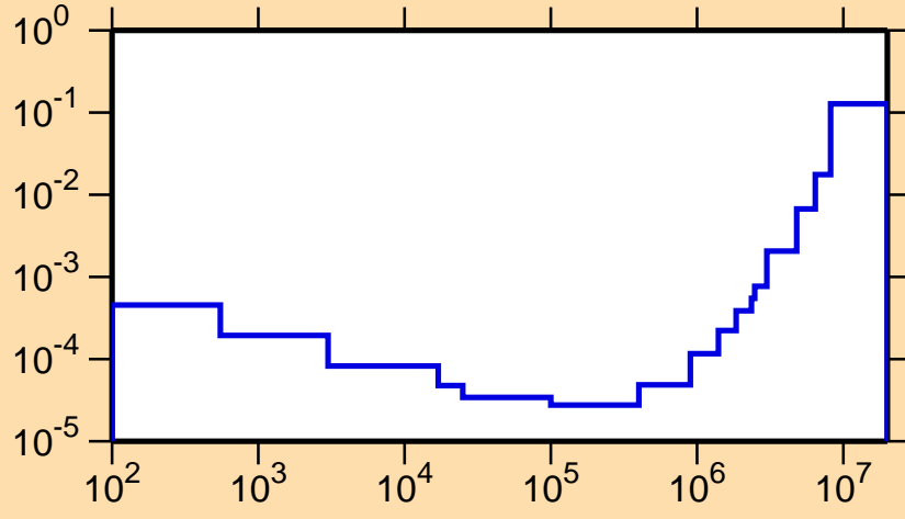
\sigma vs. E for ^{127}\text{Nd}(n,p\alpha)
