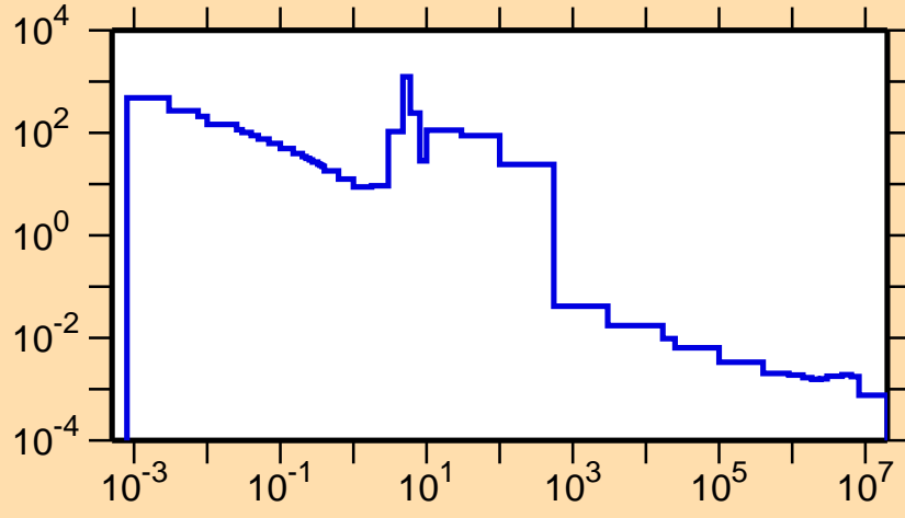
\sigma vs. E for ^{127}\text{Nd}(n,\gamma)
