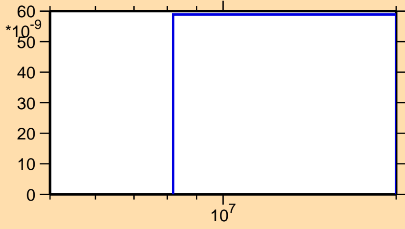
\sigma vs. E for ^{127}\text{Nd}(\text{mt117})
