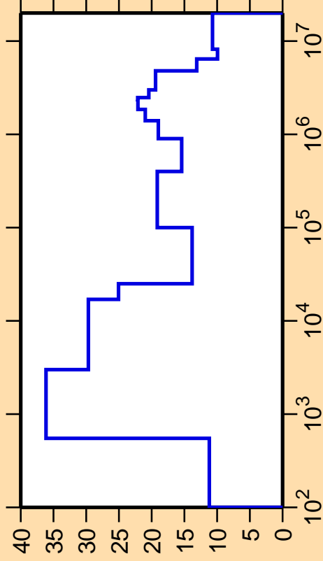
\Delta\sigma/\sigma vs. E for ^{127}\text{Nd}(n,\text{nonel.})
