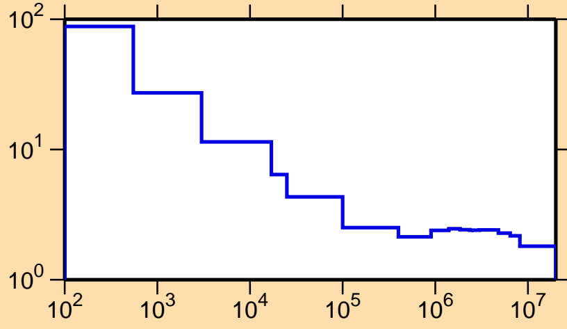
\sigma vs. E for ^{127}\text{Nd}(n,\text{nonel.})
