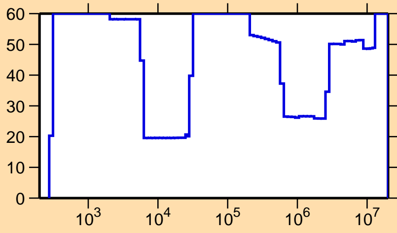
\Delta\sigma/\sigma vs. E for ^{128}\text{Nd}(n,p)
