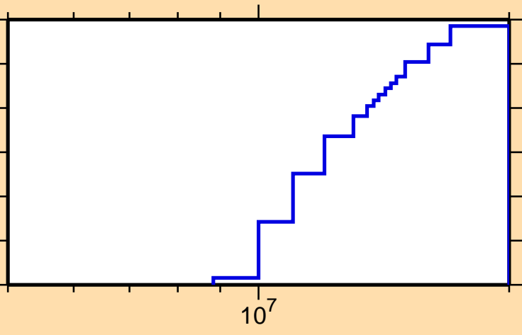
\sigma vs. E for ^{128}\text{Nd}(\text{mt117})
