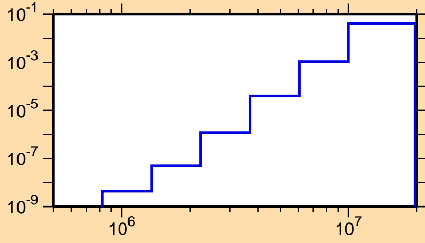
\sigma vs. E for ^{128}\text{Nd}(n,p\alpha)
