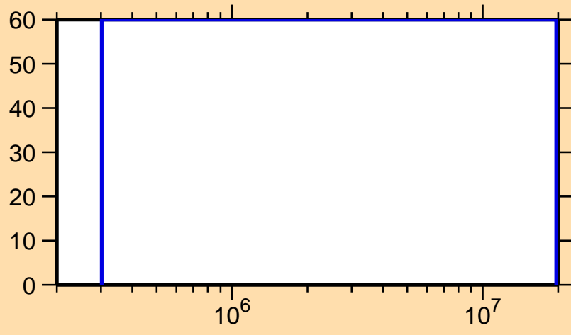
\Delta\sigma/\sigma vs. E for ^{128}\text{Nd}(n,n\text{cont.})
