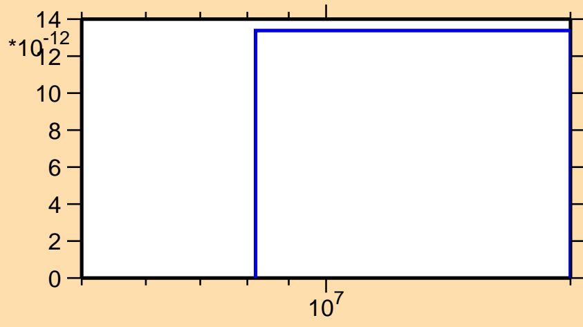
\sigma vs. E for ^{128}\text{Nd}(\text{mt } 34)
