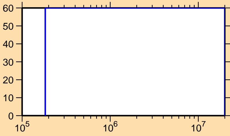
\Delta\sigma/\sigma vs. E for ^{129}\text{Nd}(n,n\text{cont.})
