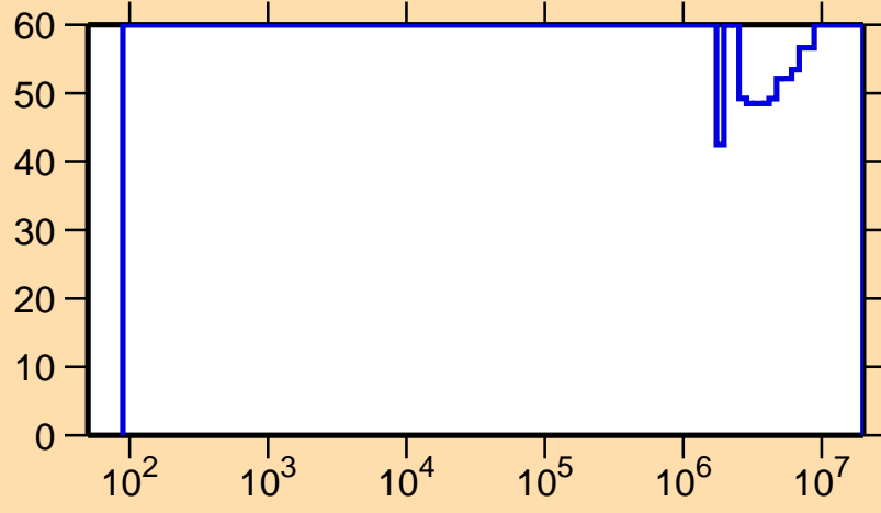
\Delta\sigma/\sigma vs. E for ^{129}\text{Nd}(n,p)
