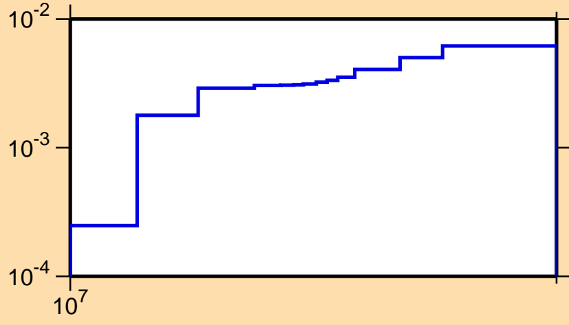
\sigma vs. E for ^{129}\text{Nd}(n,2n)
