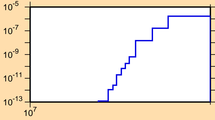
\sigma vs. E for ^{129}\text{Nd}(n,\text{nd})
