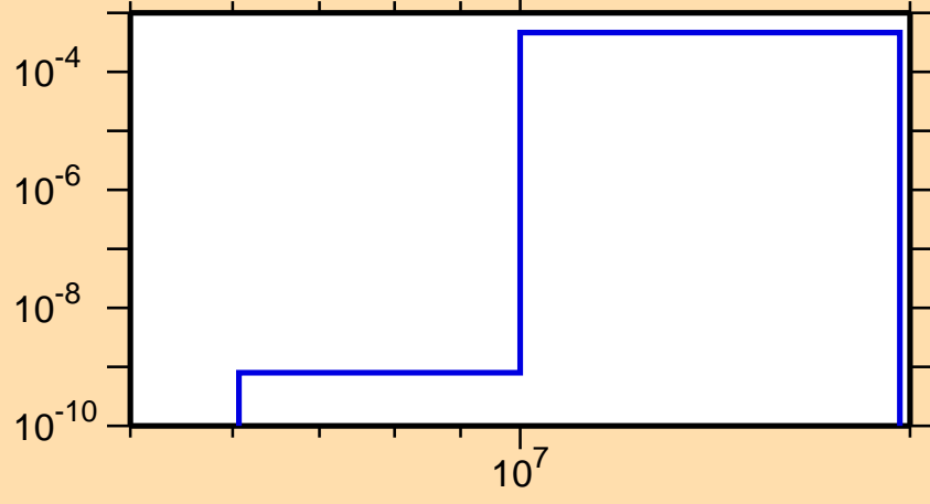
\sigma vs. E for ^{129}\text{Nd}(n,\text{pd})
