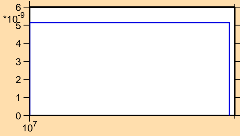
\sigma vs. E for ^{129}\text{Nd} (mt 34)
