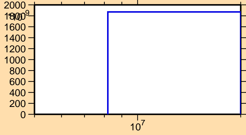
\sigma vs. E for ^{129}\text{Nd} (mt 45)
