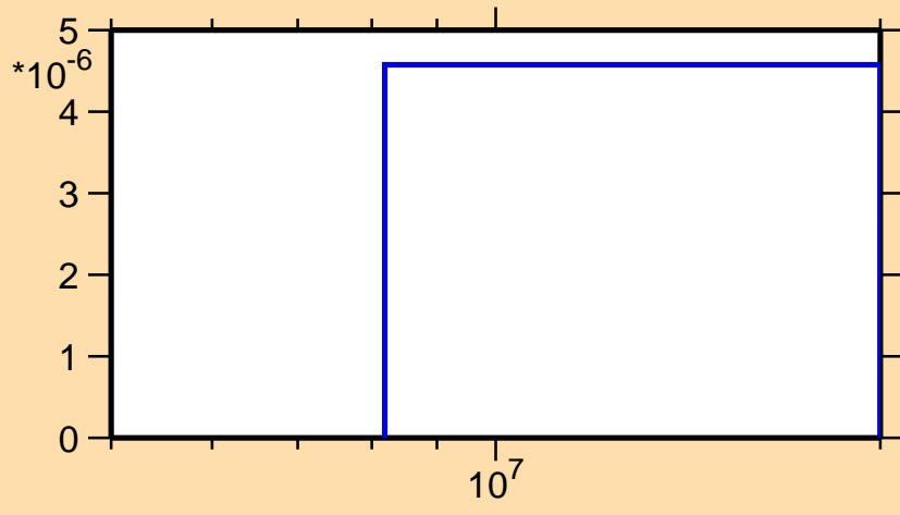
\sigma vs. E for ^{129}\text{Nd}(n,2np)
