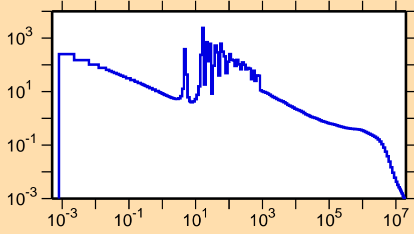
\sigma vs. E for ^{130}\text{Nd}(n,\gamma)
