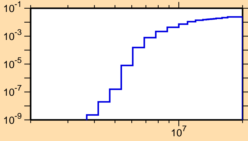
\sigma vs. E for ^{130}\text{Nd}(n,n\alpha)
