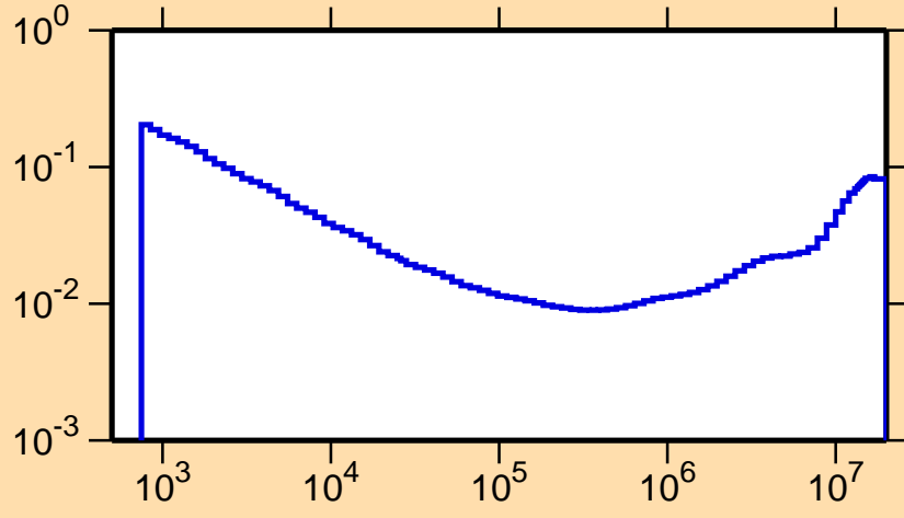
\sigma vs. E for ^{130}\text{Nd}(n,\alpha)
