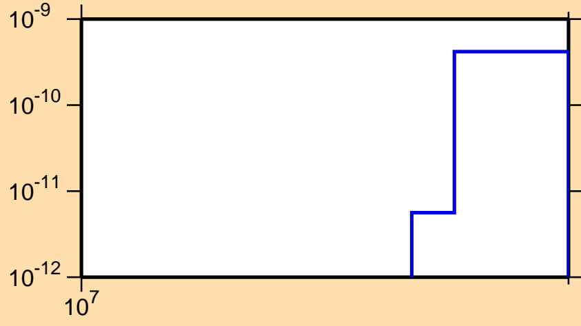
\sigma vs. E for ^{130}\text{Nd} (mt 34)
