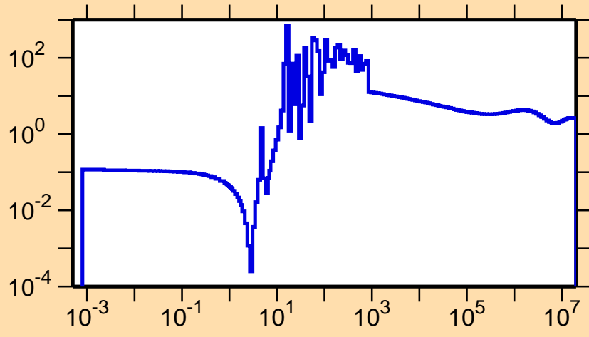
\sigma vs. E for ^{130}\text{Nd}(n,\text{el.})
