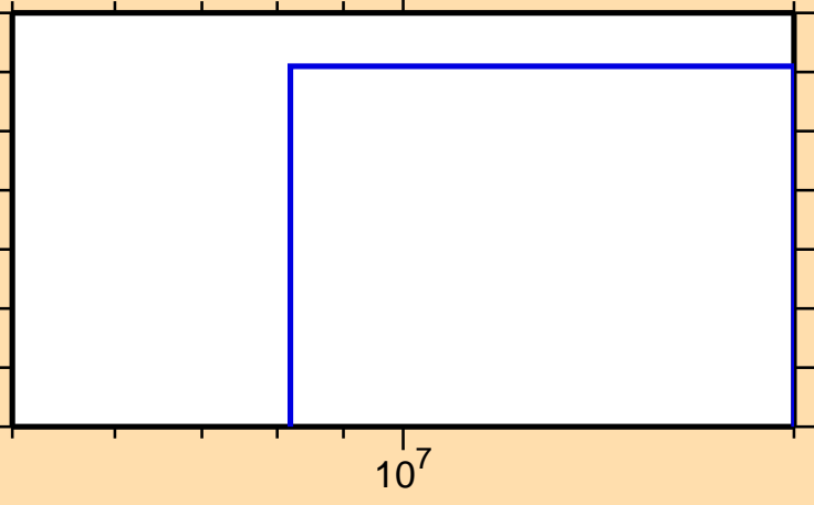
\sigma vs. E for ^{130}\text{Nd}(n,\text{pt})
