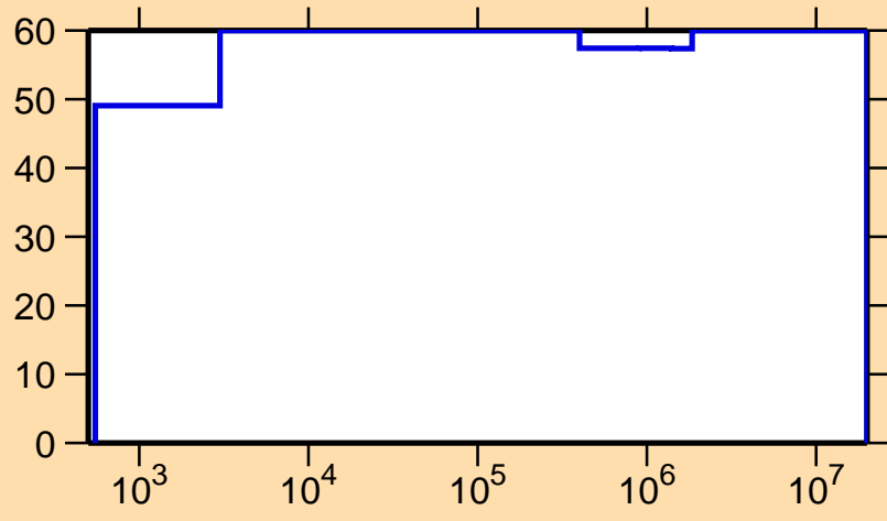
\Delta\sigma/\sigma vs. E for ^{130}\text{Nd}(n,\gamma)
