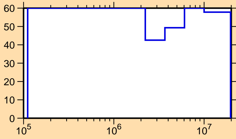
\Delta\sigma/\sigma vs. E for ^{131}\text{Nd}(n,n_1)
