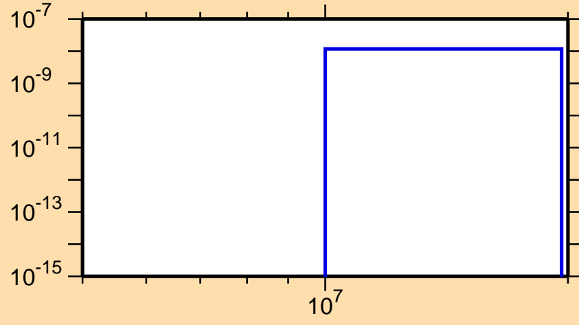
\sigma vs. E for ^{131}\text{Nd}(\text{mt117})
