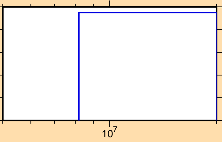
\sigma vs. E for ^{131}\text{Nd}(n,\text{nd})
