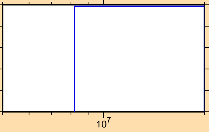
\sigma vs. E for ^{131}\text{Nd} (mt 45)
