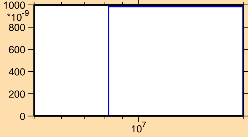
\sigma vs. E for ^{131}\text{Nd} (mt 45)
