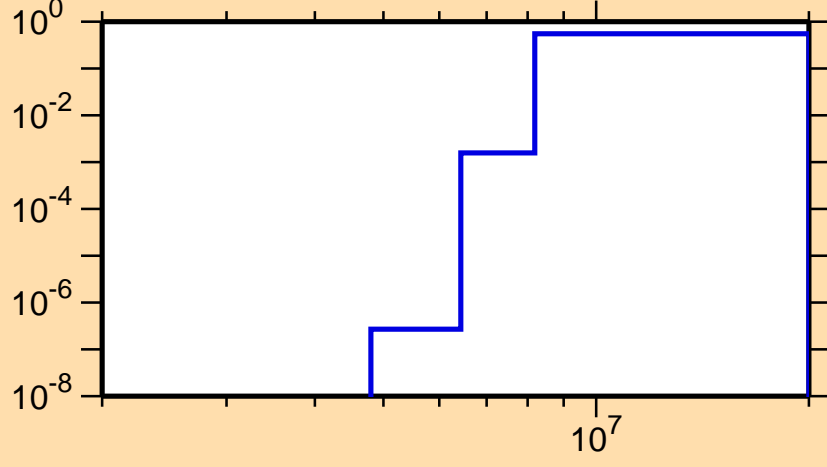
\sigma vs. E for ^{131}\text{Nd}(n,np)
