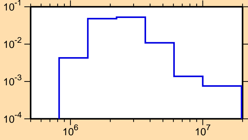
\sigma vs. E for ^{132}\text{Nd}(n,n_4)
