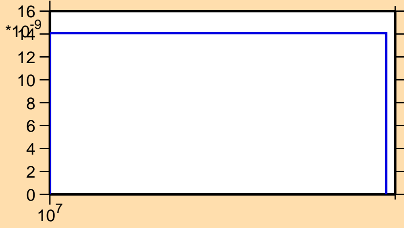
\sigma vs. E for ^{132}\text{Nd}(n,2np)
