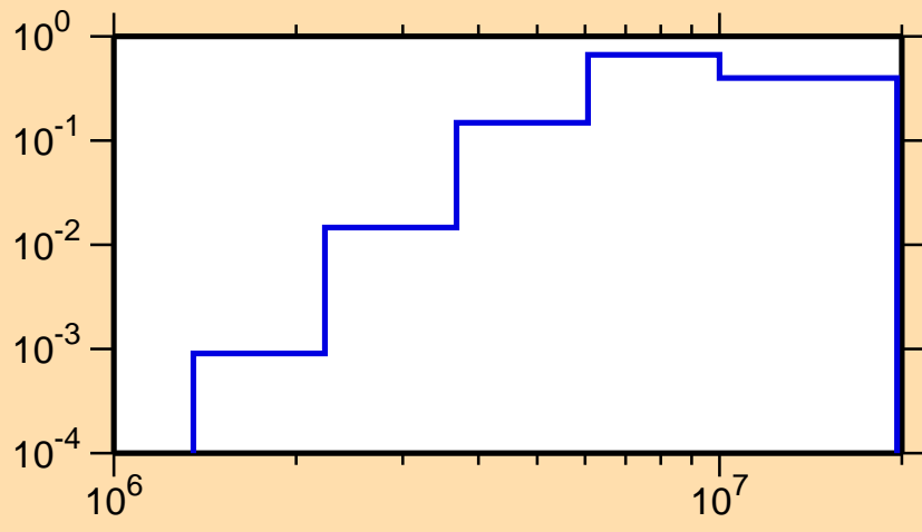
\sigma vs. E for ^{132}\text{Nd}(n,n\text{cont.})
