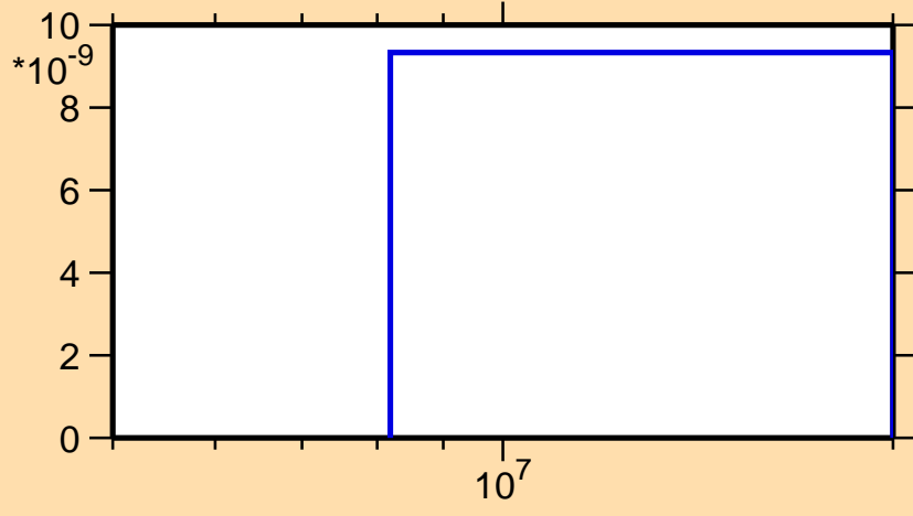
\sigma vs. E for ^{132}\text{Nd}(\text{mt117})
