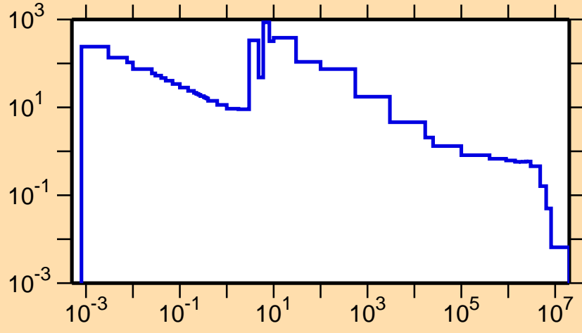
\sigma vs. E for ^{132}\text{Nd}(n,\gamma)
