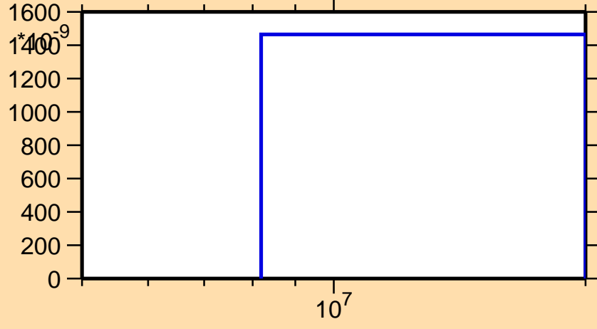
\sigma vs. E for ^{132}\text{Nd}(\text{mt } 45)
