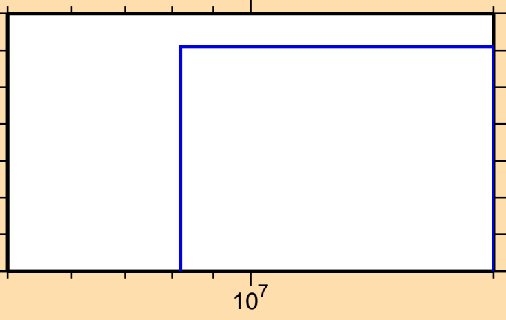
\sigma vs. E for ^{132}\text{Nd}(n,\text{pd})
