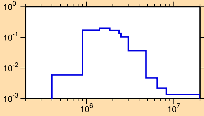
\sigma vs. E for ^{132}\text{Nd}(n,n_3)
