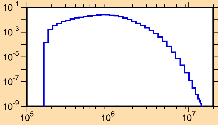
\sigma vs. E for ^{133}\text{Nd}(n,n_2)
