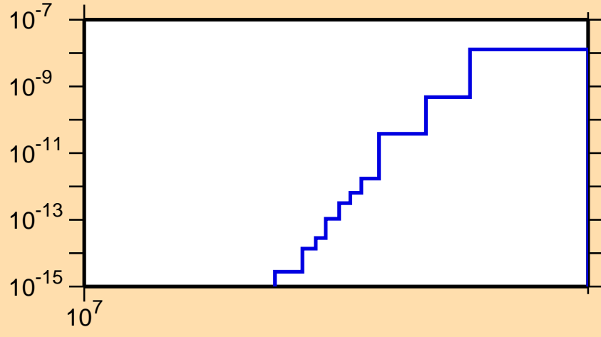
\sigma vs. E for ^{133}\text{Nd} (mt 34)
