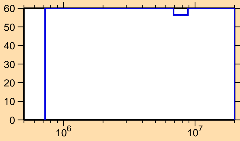
\Delta\sigma/\sigma vs. E for ^{133}\text{Nd}(n,n\text{cont.})
