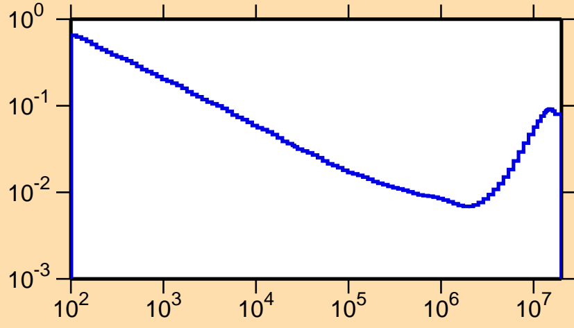
\sigma vs. E for ^{133}\text{Nd}(n,\alpha)
