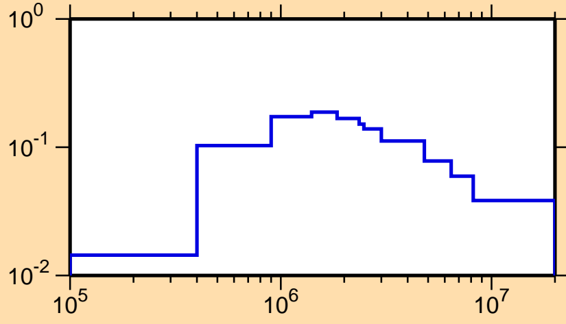
\sigma vs. E for ^{133}\text{Nd}(n,n_4)
