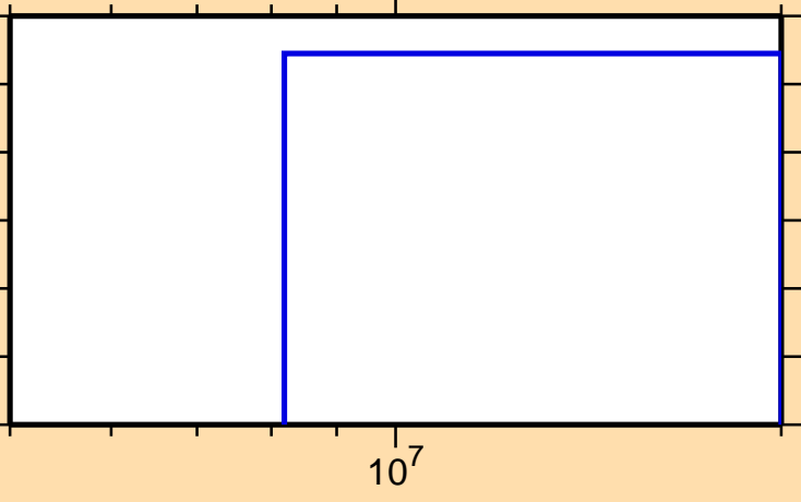
\sigma vs. E for ^{133}\text{Nd}(\text{mt } 45)
