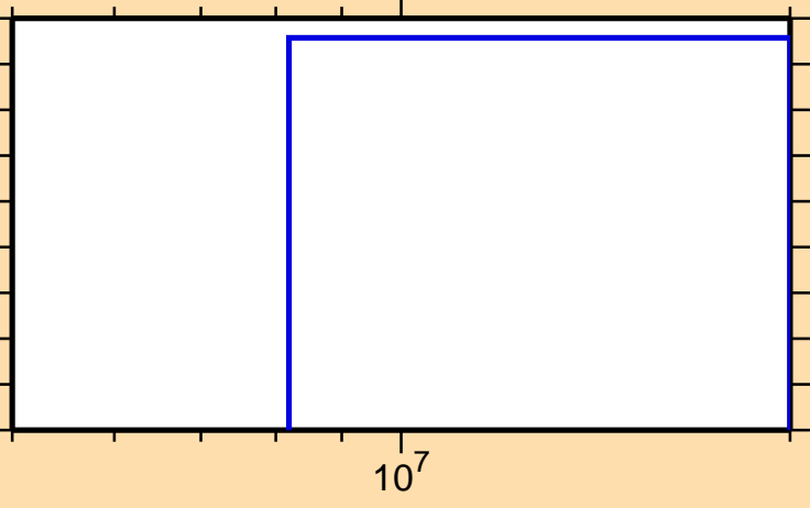
\sigma vs. E for ^{133}\text{Nd}(n,2np)
