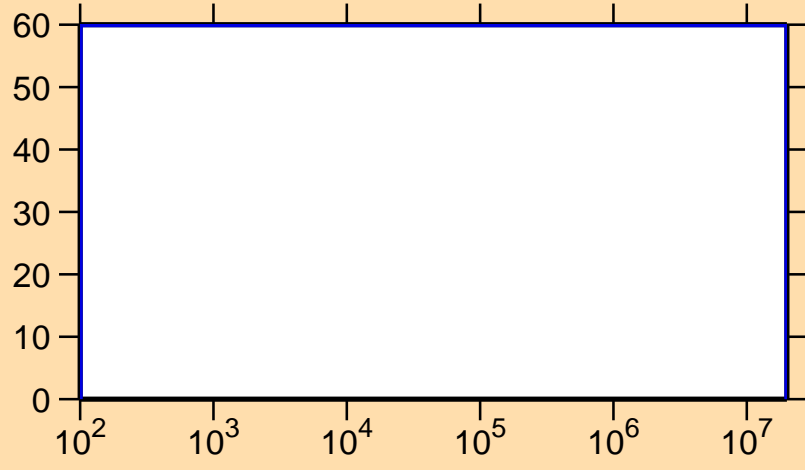
\Delta\sigma/\sigma vs. E for ^{133}\text{Nd}(n,\gamma)
