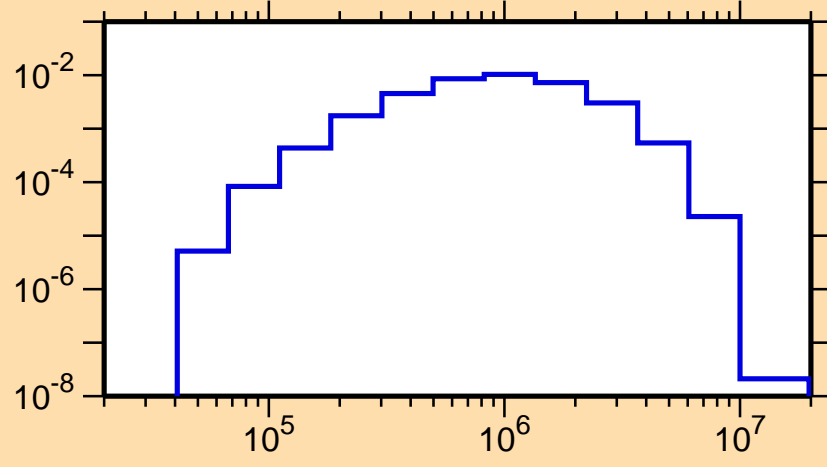
\sigma vs. E for ^{133}\text{Nd}(n,n_3)
