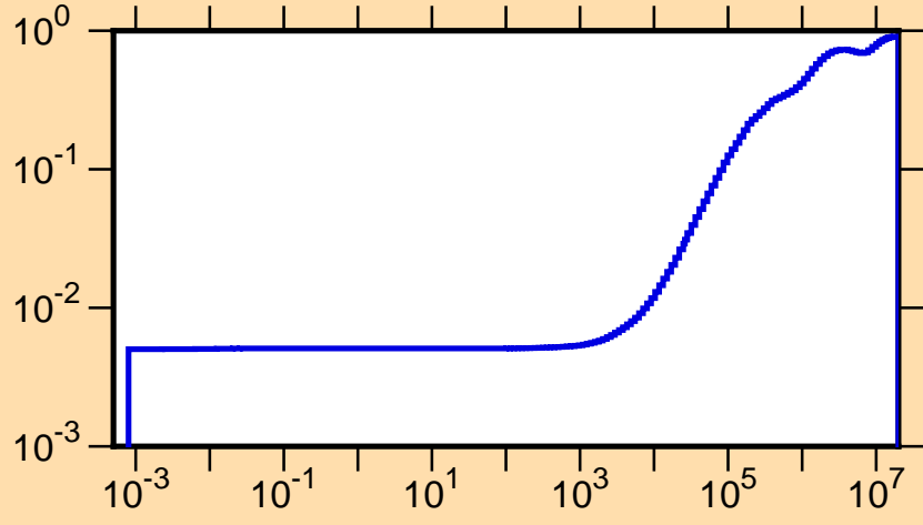
\mu vs. E for ^{134}\text{Nd}(\text{mt251})
