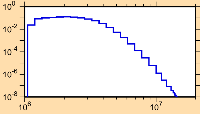
\sigma vs. E for ^{134}\text{Nd}(n,n_4)
