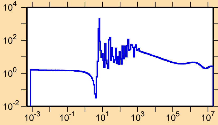
\sigma vs. E for ^{134}\text{Nd}(n,\text{el.})
