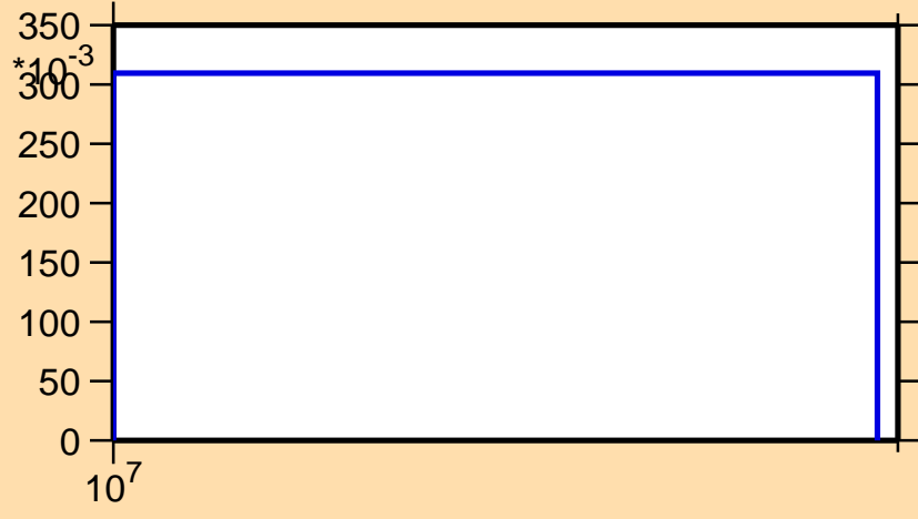
\sigma vs. E for ^{134}\text{Nd}(n,2n)
