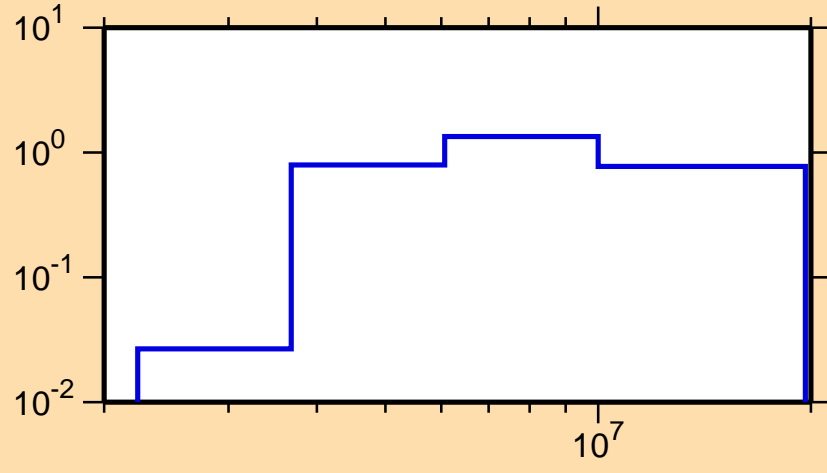
\sigma vs. E for ^{134}\text{Nd}(n,n\text{cont.})
