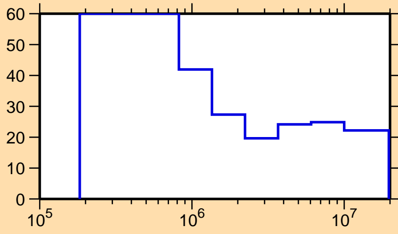
\Delta\sigma/\sigma vs. E for ^{134}\text{Nd}(n,n_1)
