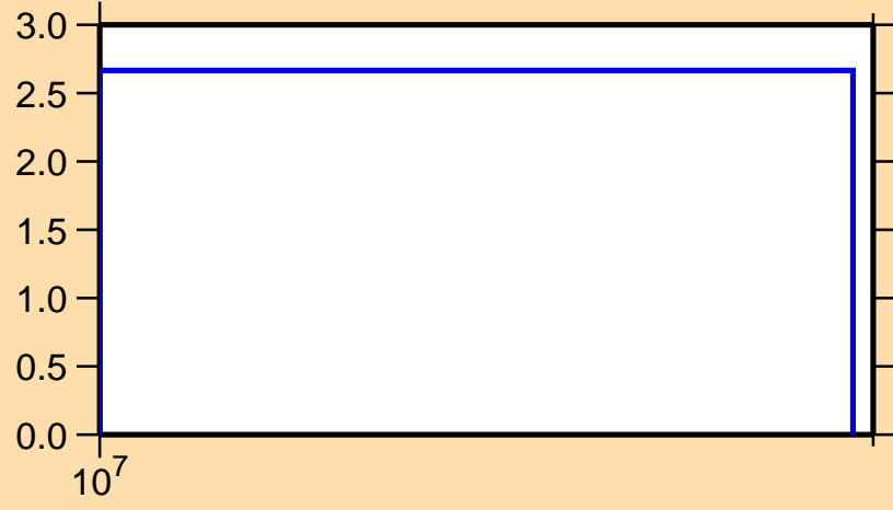
\Delta\sigma/\sigma vs. E for ^{134}\text{Nd}(n,\text{tot.})
