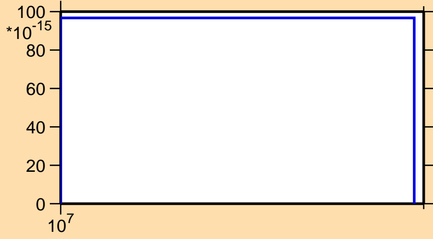
\sigma vs. E for ^{134}\text{Nd} (mt 34)
