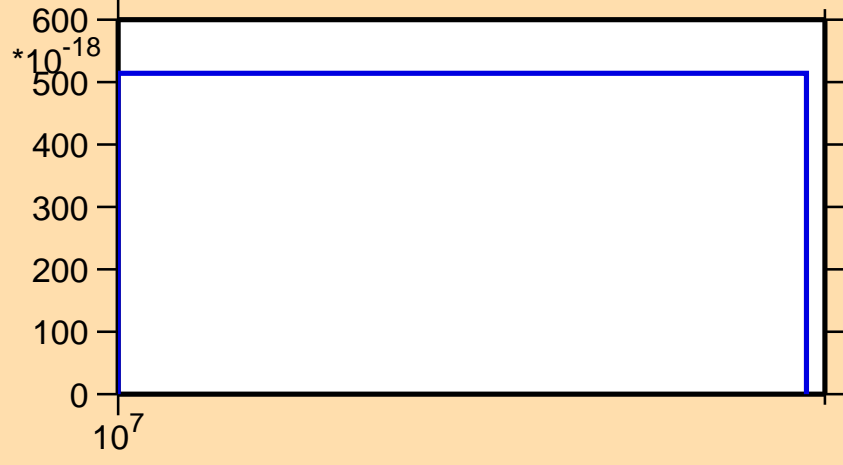
\sigma vs. E for ^{134}\text{Nd}(n,nt)
