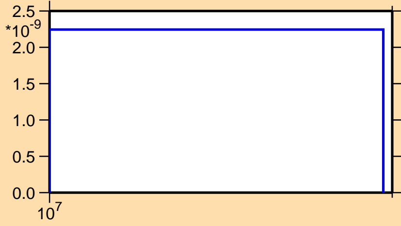
\sigma vs. E for ^{134}\text{Nd}(n,2np)
