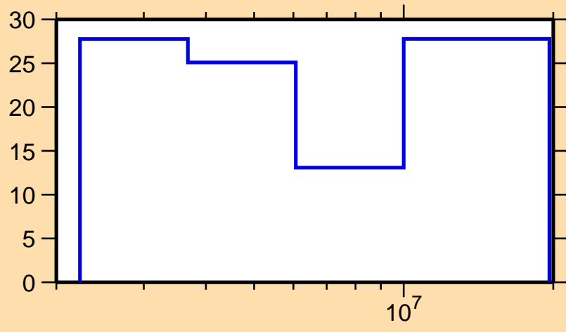
\Delta\sigma/\sigma vs. E for ^{134}\text{Nd}(n,\text{inel.})
