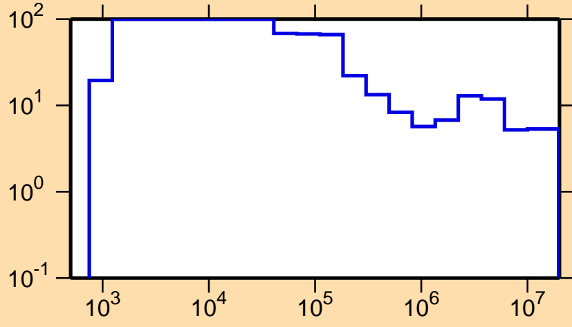
\Delta\sigma/\sigma vs. E for ^{134}\text{Nd}(n,\text{el.})
