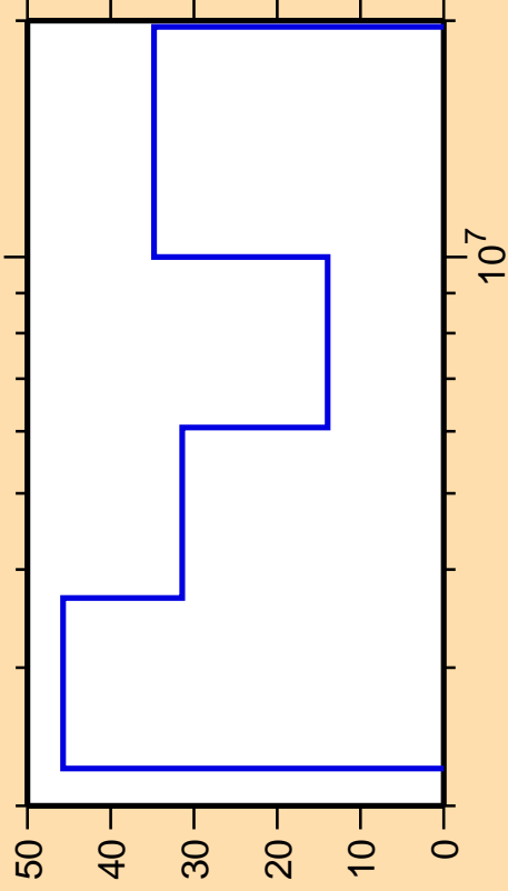
\Delta\sigma/\sigma vs. E for ^{134}\text{Nd}(n,n\text{cont.})
