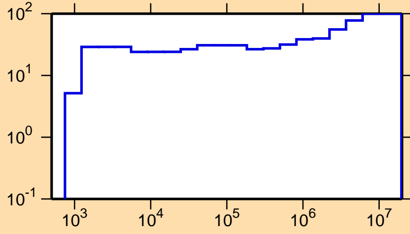
\Delta\sigma/\sigma vs. E for ^{134}\text{Nd}(n,\gamma)
