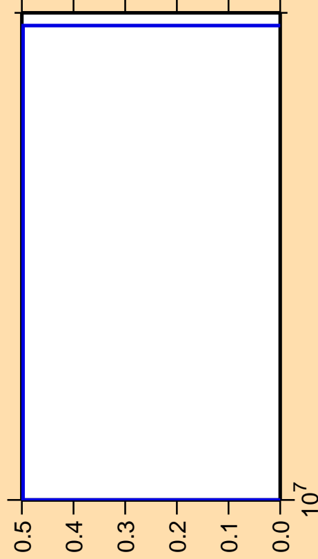
\Delta\sigma/\sigma vs. E for ^{134}\text{Nd} (mt 34)
