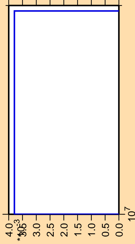
\Delta\sigma/\sigma vs. E for ^{134}\text{Nd}(n,nt)
