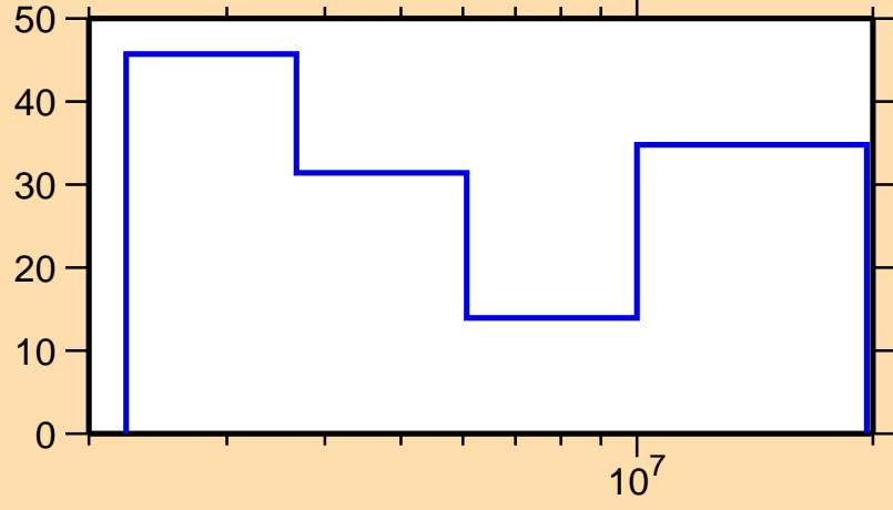
\Delta\sigma/\sigma vs. E for ^{134}\text{Nd}(n,n\text{cont.})
