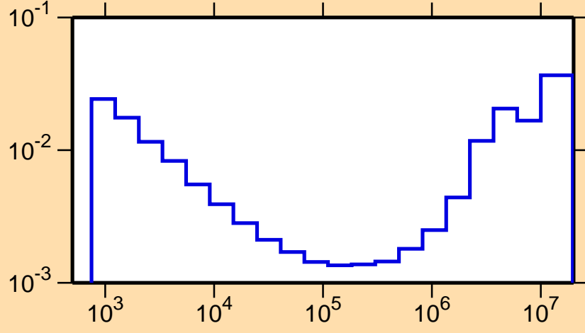
\sigma vs. E for ^{134}\text{Nd}(n,\alpha)
