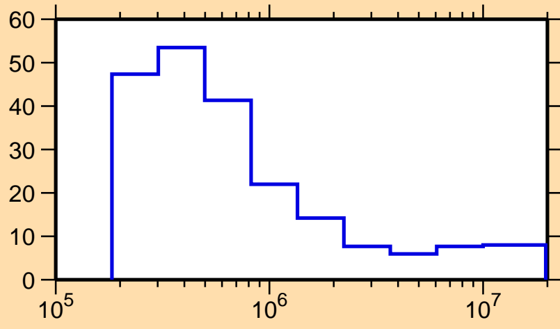
\Delta\sigma/\sigma vs. E for ^{134}\text{Nd}(n,\text{nonel.})
