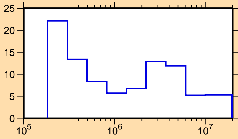
\Delta\sigma/\sigma vs. E for ^{134}\text{Nd}(n,\text{el.})
