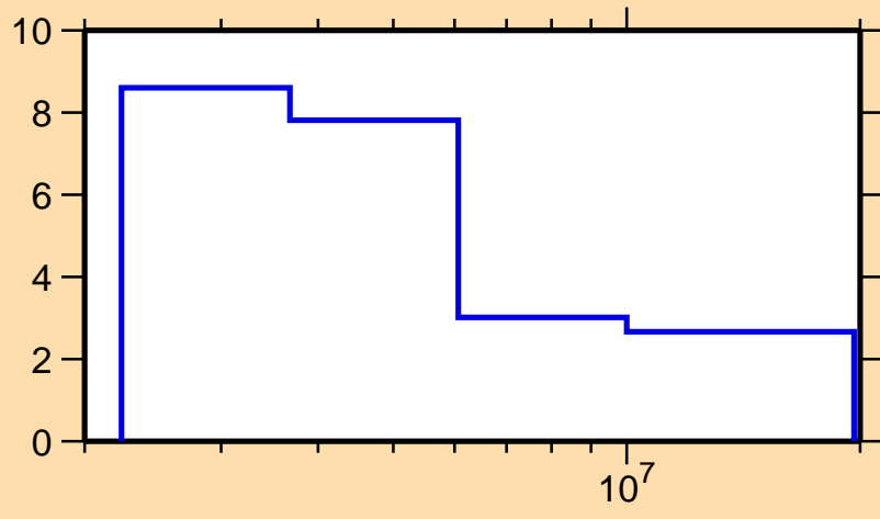
\Delta\sigma/\sigma vs. E for ^{134}\text{Nd}(n,\text{tot.})
