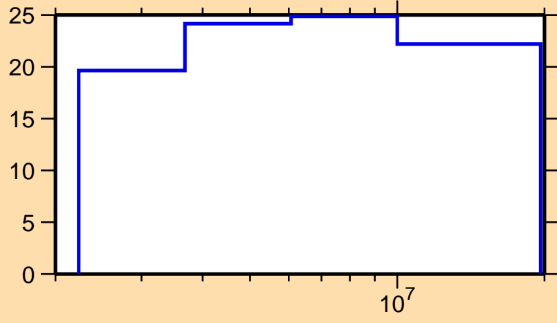
\Delta\sigma/\sigma vs. E for ^{134}\text{Nd}(n,n_1)
