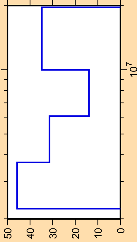
\Delta\sigma/\sigma vs. E for ^{134}\text{Nd}(n,n_{\text{cont}}) .
