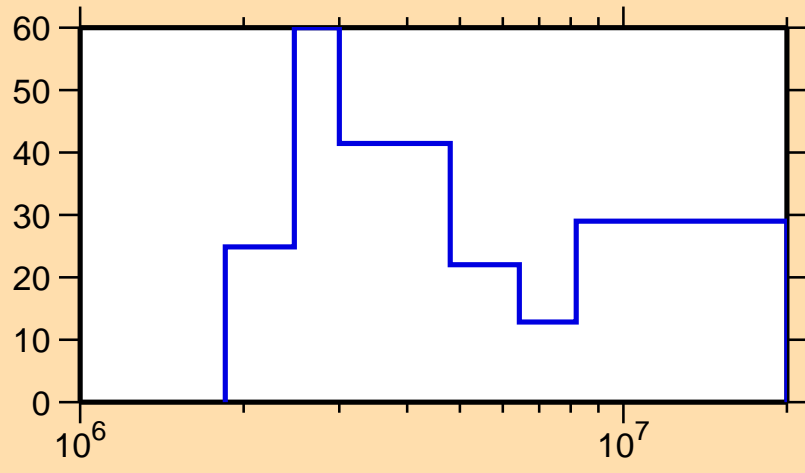
\Delta\sigma/\sigma vs. E for ^{134}\text{Nd}(n,n\text{cont.})
