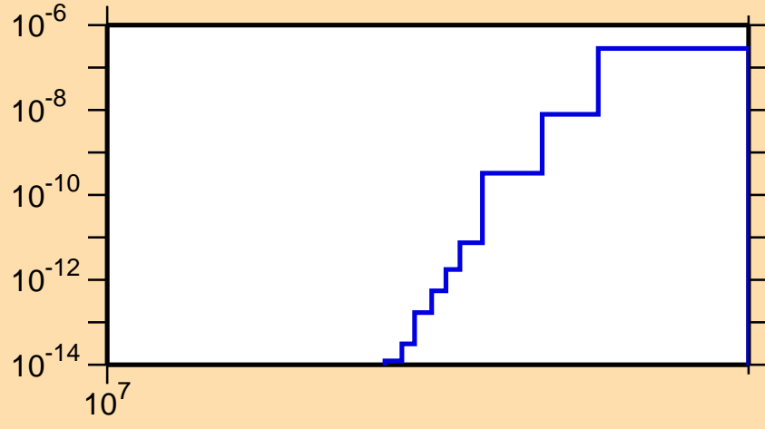
\sigma vs. E for ^{135}\text{Nd}(n,\text{pt})
