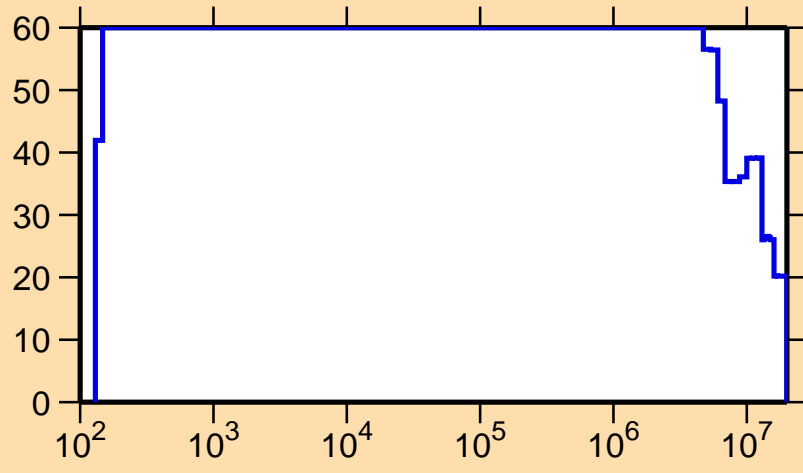
\Delta\sigma/\sigma vs. E for ^{135}\text{Nd}(n,p)
