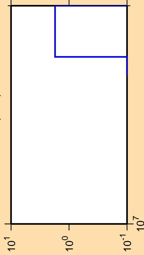
\Delta\sigma/\sigma vs. E for ^{135}\text{Nd}(n,nt)
