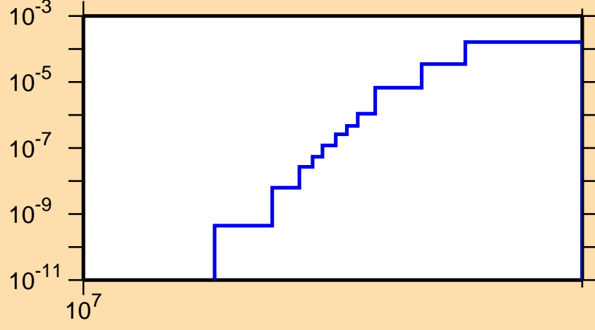
\sigma vs. E for ^{135}\text{Nd}(n,2n\alpha)
