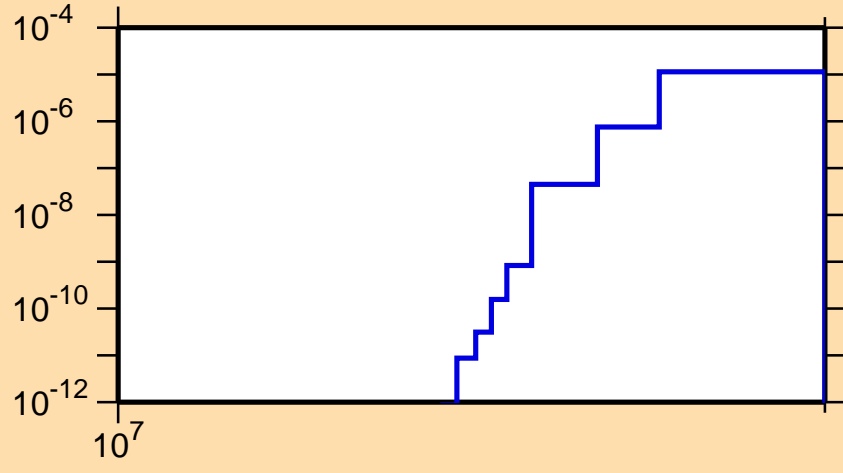
\sigma vs. E for ^{135}\text{Nd}(n,\text{nd})
