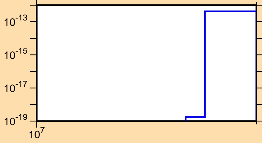
\sigma vs. E for ^{135}\text{Nd}(n,nt)
