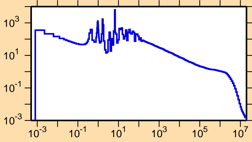
\sigma vs. E for ^{135}\text{Nd}(n,\gamma)
