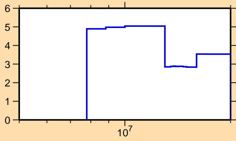
\Delta\sigma/\sigma vs. E for ^{135}\text{Nd}(n,\text{el.})
