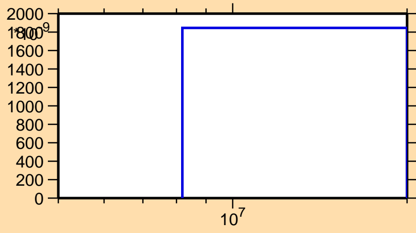
\sigma vs. E for ^{135}\text{Nd}(n,\text{He3})
