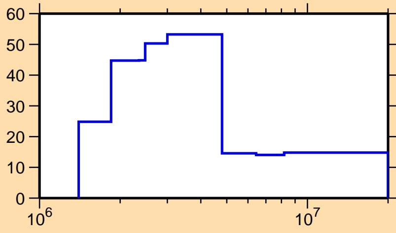
\Delta\sigma/\sigma vs. E for ^{135}\text{Nd}(n,n_1)
