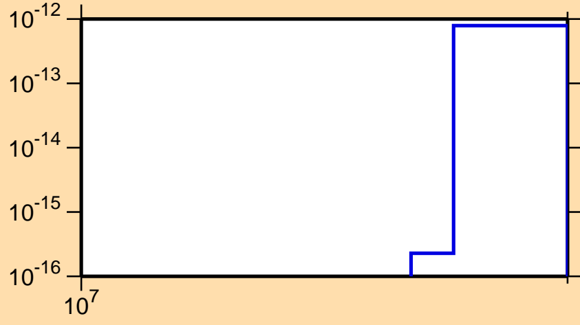
\sigma vs. E for ^{136}\text{Nd} (mt 34)
