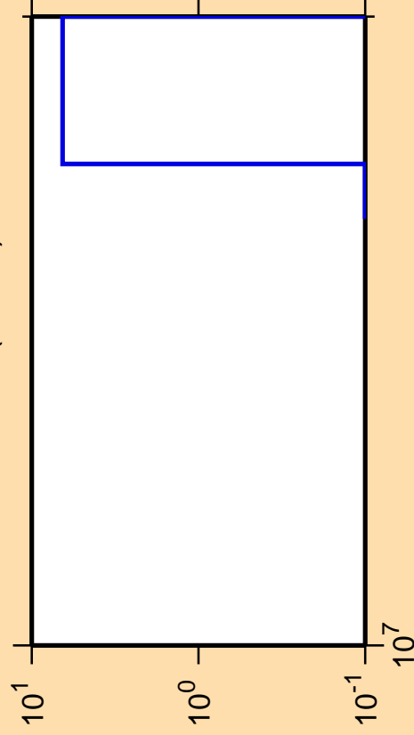
\Delta\sigma/\sigma vs. E for ^{136}\text{Nd} (mt 34)
