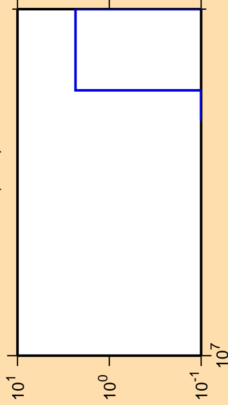
\Delta\sigma/\sigma vs. E for ^{136}\text{Nd}(n,nt)
