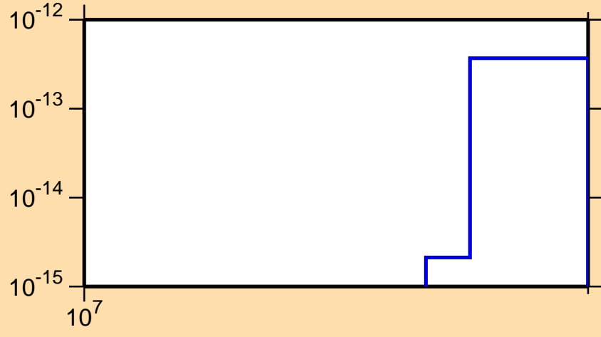
\sigma vs. E for ^{136}\text{Nd}(n,nt)
