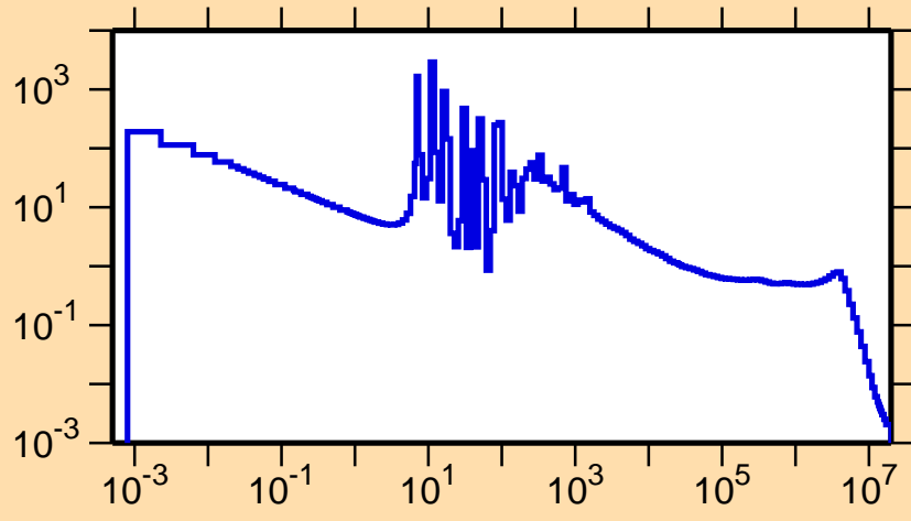
\sigma vs. E for ^{136}\text{Nd}(n,\gamma)
