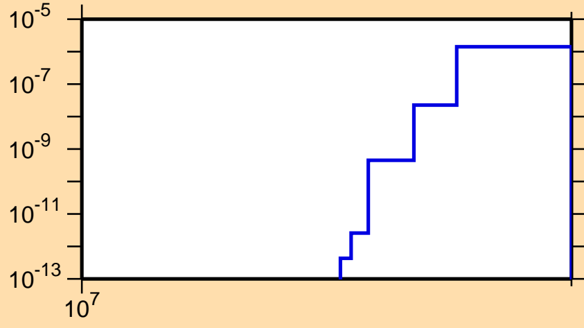
\sigma vs. E for ^{136}\text{Nd}(n,2n\alpha)
