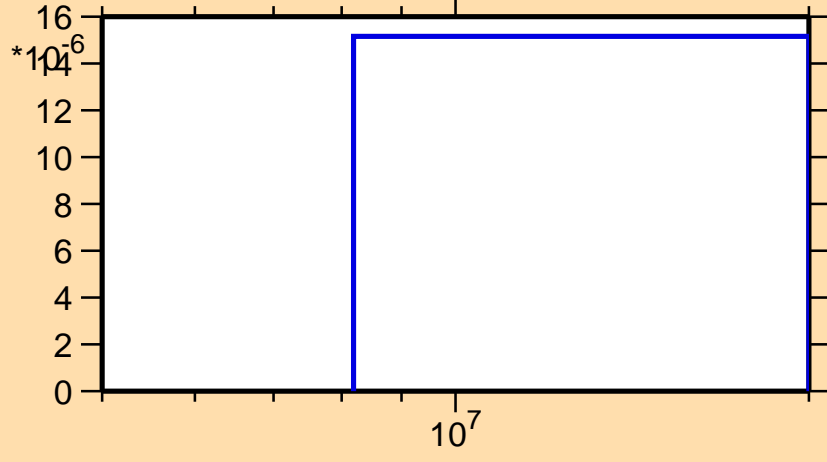
\sigma vs. E for ^{136}\text{Nd}(n,t)
