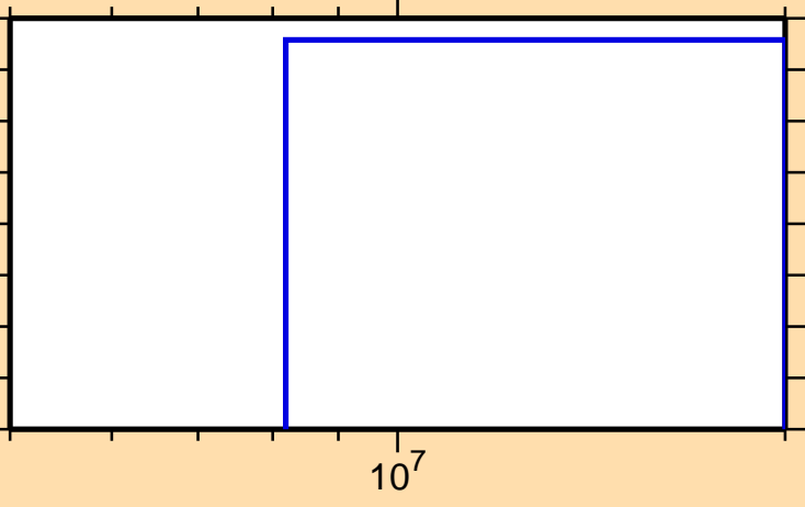
\sigma vs. E for ^{136}\text{Nd}(n,t)
