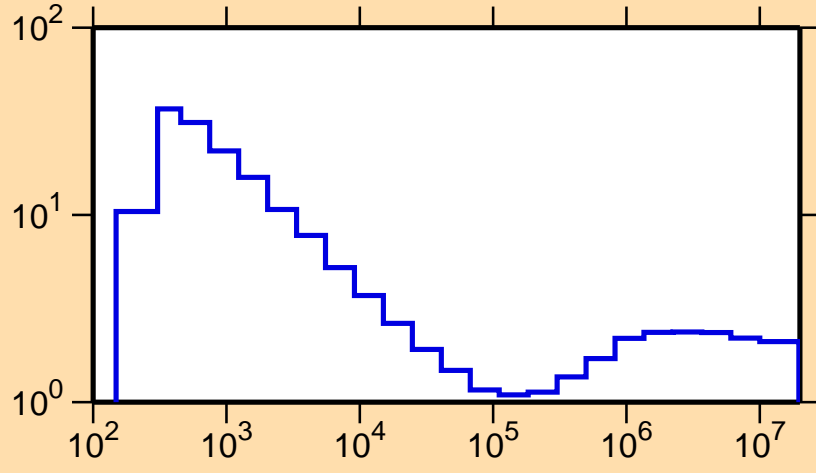
\sigma vs. E for ^{137}\text{Nd}(n,\text{nonel.})
