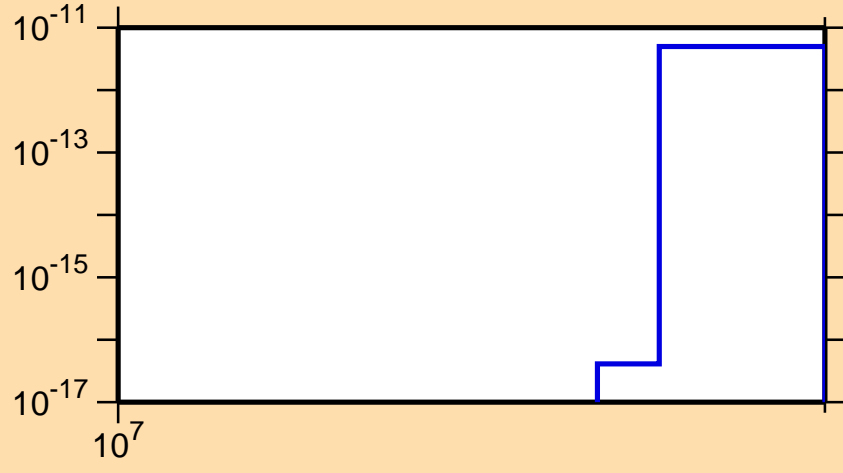
\sigma vs. E for ^{137}\text{Nd}(n,nt)
