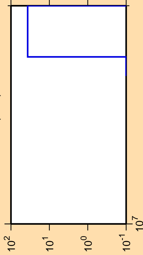
\Delta\sigma/\sigma vs. E for ^{137}\text{Nd}(n,nt)
