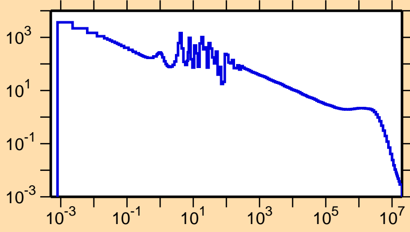
\sigma vs. E for ^{137}\text{Nd}(n,\gamma)
