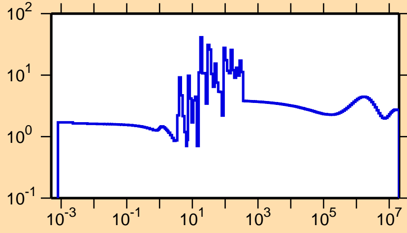
\sigma vs. E for ^{137}\text{Nd}(n,\text{el.})
