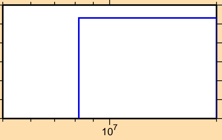
\sigma vs. E for ^{137}\text{Nd}(\text{mt117})
