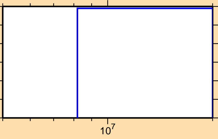
\sigma vs. E for ^{137}\text{Nd}(n,\text{nd})
