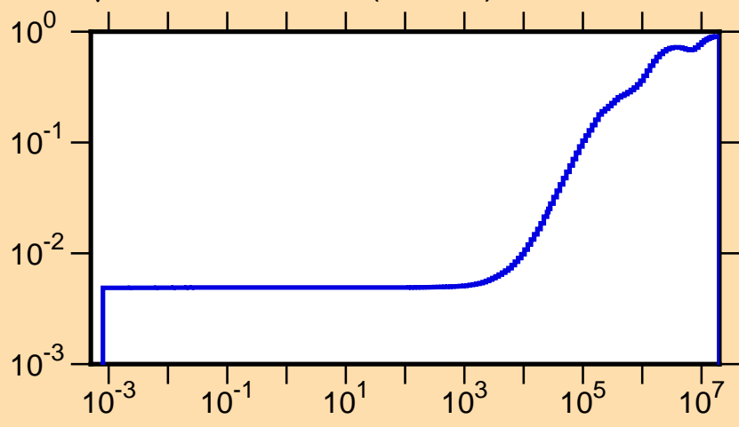
\mu vs. E for ^{138}\text{Nd}(\text{mt251})
