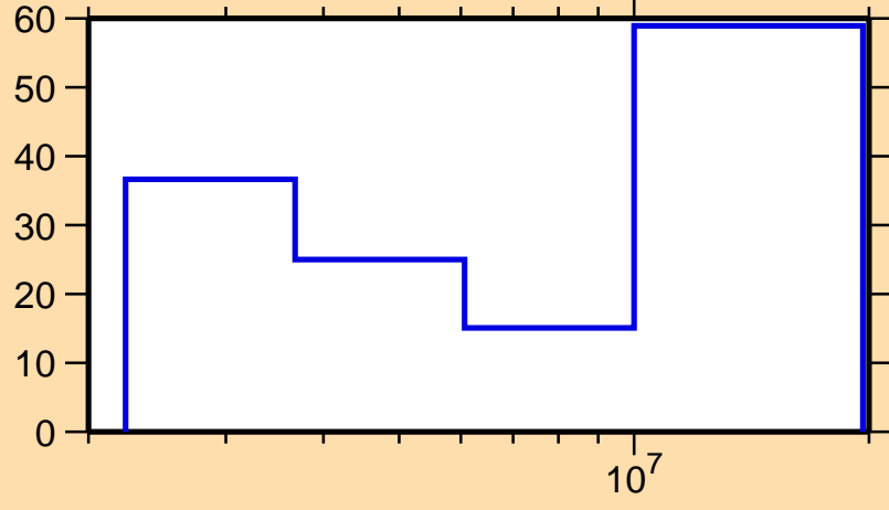
\Delta\sigma/\sigma vs. E for ^{138}\text{Nd}(n,n\text{cont.})
