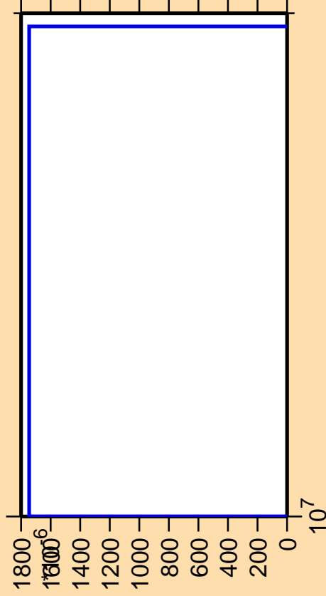
\Delta\sigma/\sigma vs. E for ^{138}\text{Nd} (mt 34)
