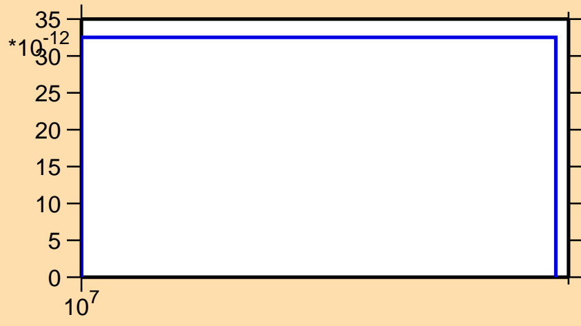
\sigma vs. E for ^{138}\text{Nd}(\text{mt } 45)
