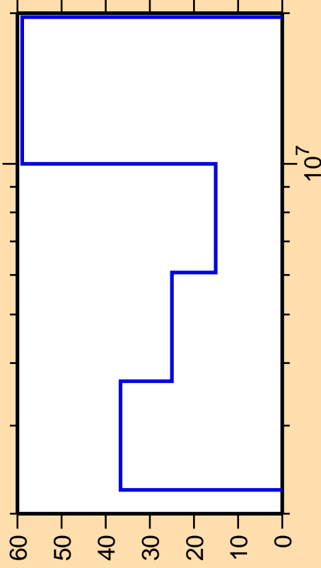
\Delta\sigma/\sigma vs. E for ^{138}\text{Nd}(n,n\text{cont.})
