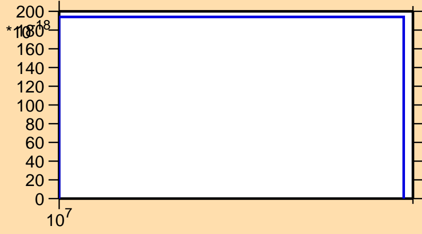
\sigma vs. E for ^{138}\text{Nd} (mt 34)
