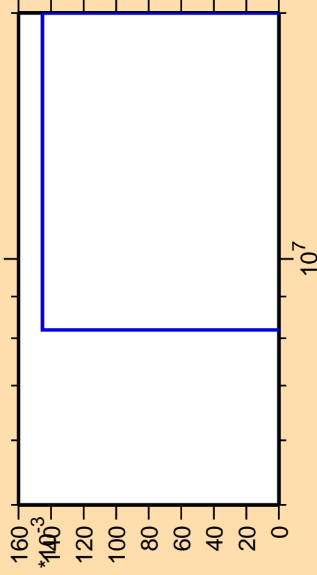
\Delta\sigma/\sigma vs. E for ^{138}\text{Nd}(n,nt)
