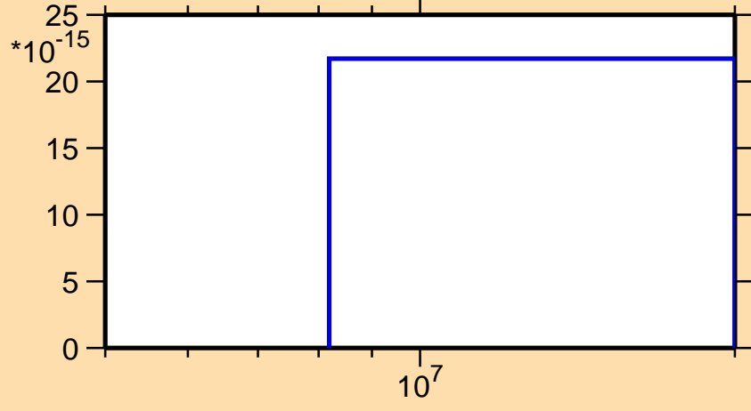
\sigma vs. E for ^{138}\text{Nd}(n,nt)
