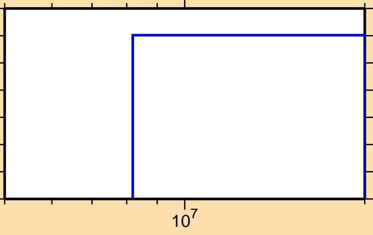
\sigma vs. E for ^{138}\text{Nd}(n,2np)
