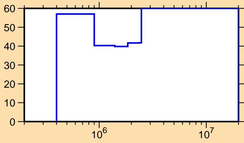
\Delta\sigma/\sigma vs. E for ^{138}\text{Nd}(n,n_1)
