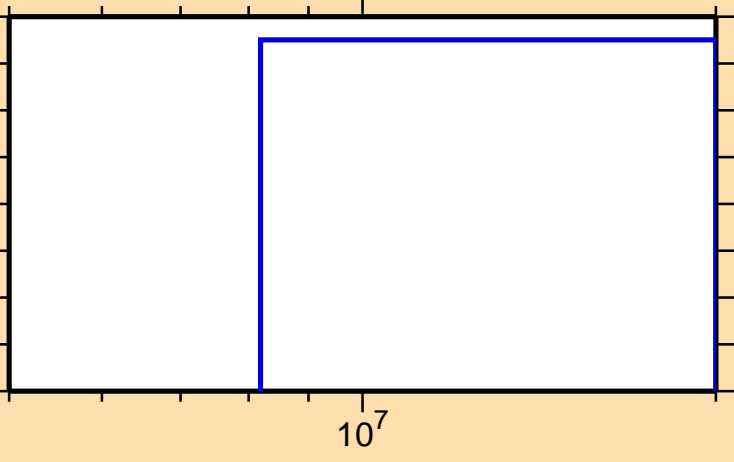
\sigma vs. E for ^{138}\text{Nd}(n,t)
