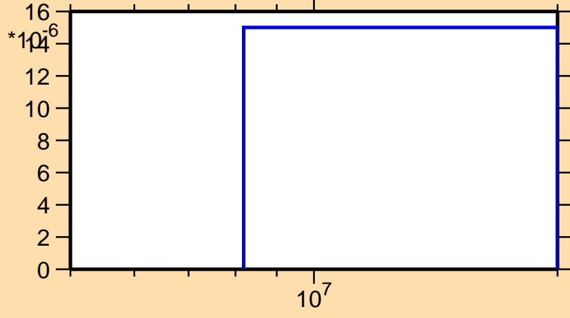
\sigma vs. E for ^{138}\text{Nd}(n,t)
