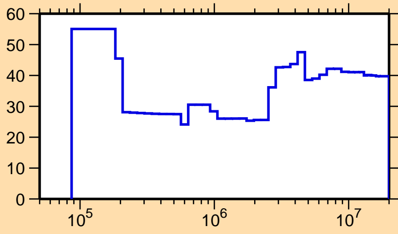
\Delta\sigma/\sigma vs. E for ^{139}\text{Nd}(n,n_1)
