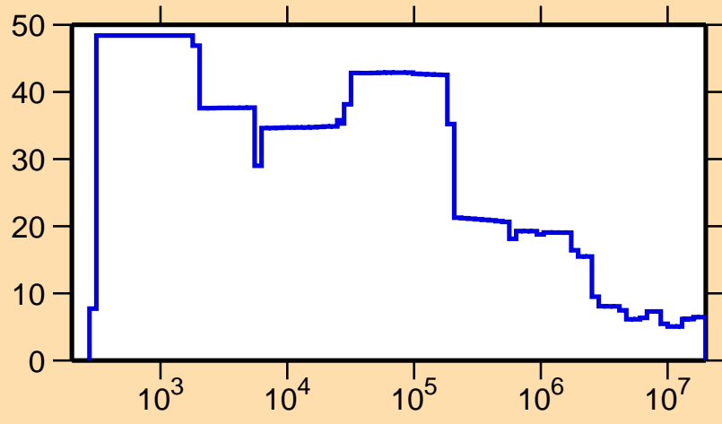
\Delta\sigma/\sigma vs. E for ^{139}\text{Nd}(n,\text{nonel.})
