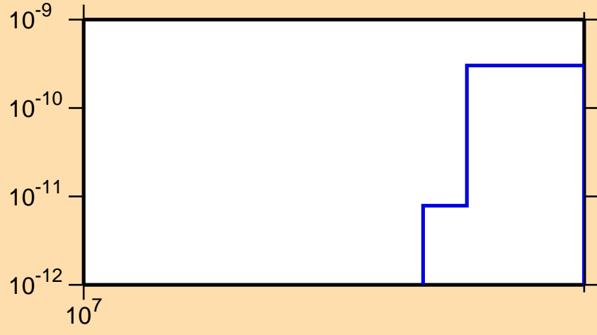
\sigma vs. E for ^{139}\text{Nd} (mt 45)
