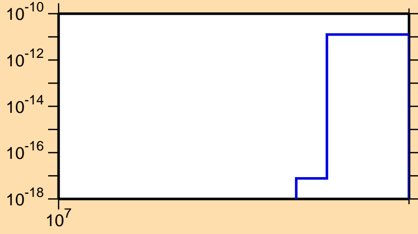
\sigma vs. E for ^{139}\text{Nd}(n,nt)
