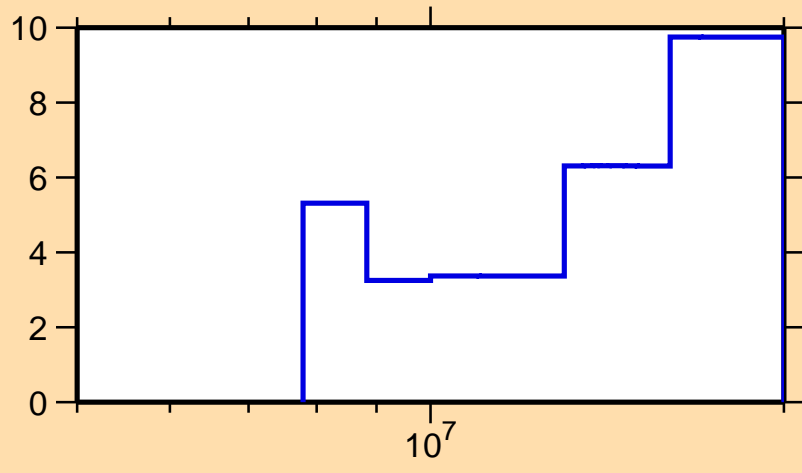
\Delta\sigma/\sigma vs. E for ^{139}\text{Nd}(n,\text{tot.})
