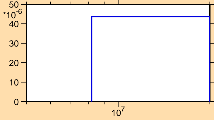
\sigma vs. E for ^{139}\text{Nd}(n,t)
