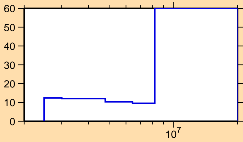
\Delta\sigma/\sigma vs. E for ^{139}\text{Nd}(n,n\text{cont.})
