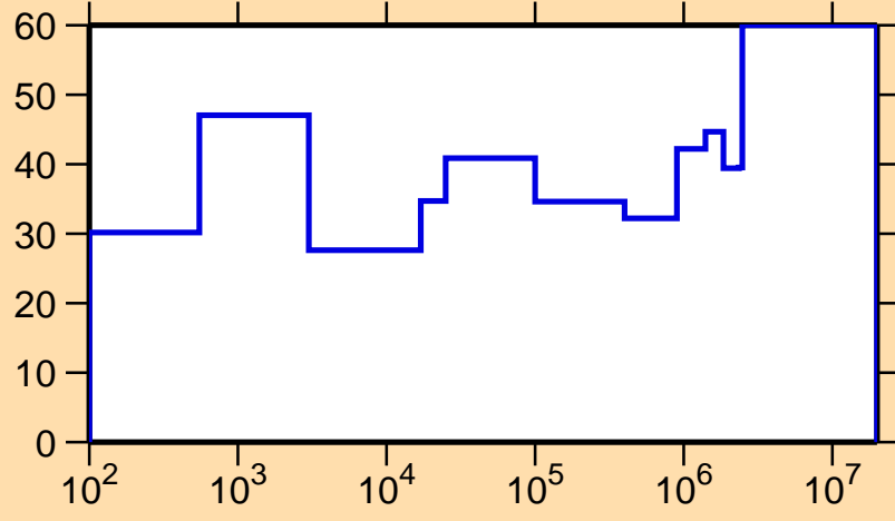
\Delta\sigma/\sigma vs. E for ^{139}\text{Nd}(n,\gamma)
