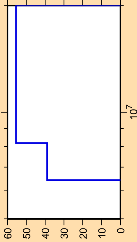
\Delta\sigma/\sigma vs. E for ^{139}\text{Nd}(n,p)
