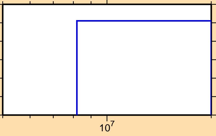
\sigma vs. E for ^{139}\text{Nd}(n,\text{pt})
